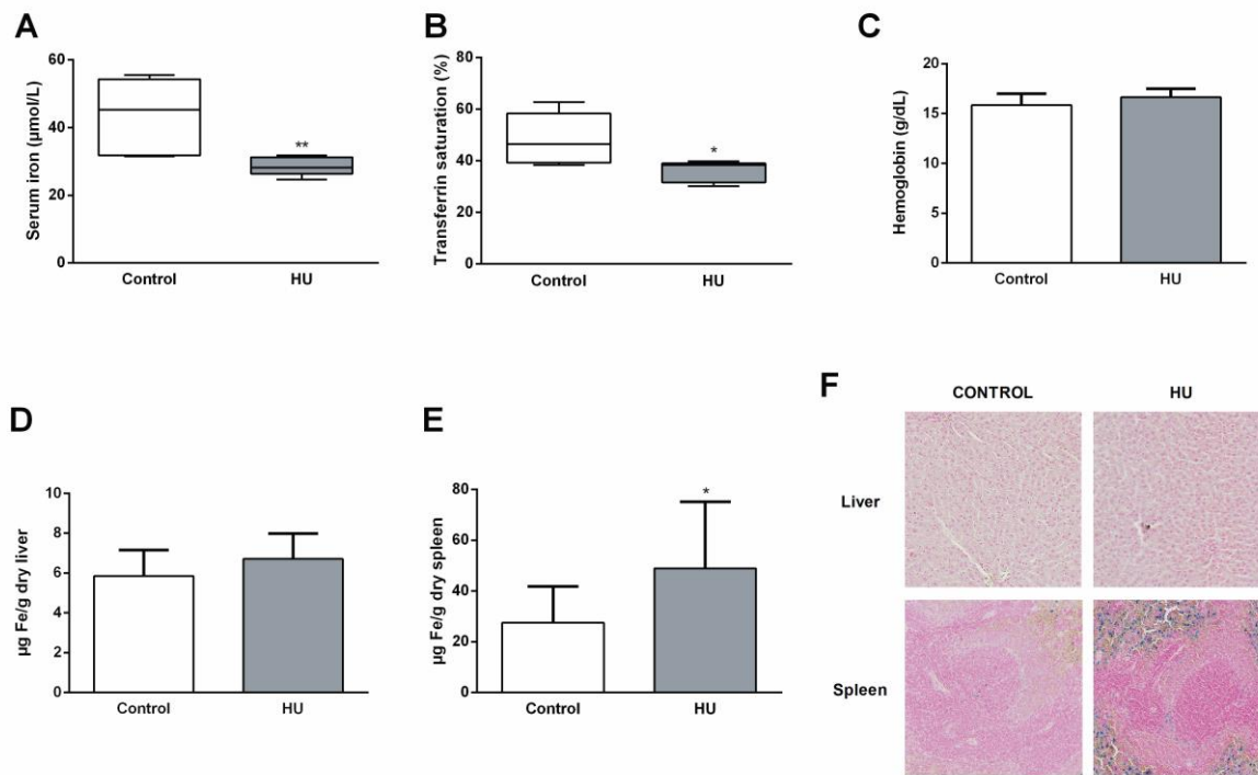
Figure 1. Hindlimb unloading induces iron misdistribution. A: Serum iron concentration. B: transferrin saturation. C: hemoglobin concentration. D: liver iron concentration. E: spleen iron concentration. F: histological detection of iron deposits in liver and spleen sections by Perls' iron staining. Significance was checked using Mann-Whitney (A and B) or unpaired t-test (C, D, E). * p < 0.05 , ** p < 0.01 .
