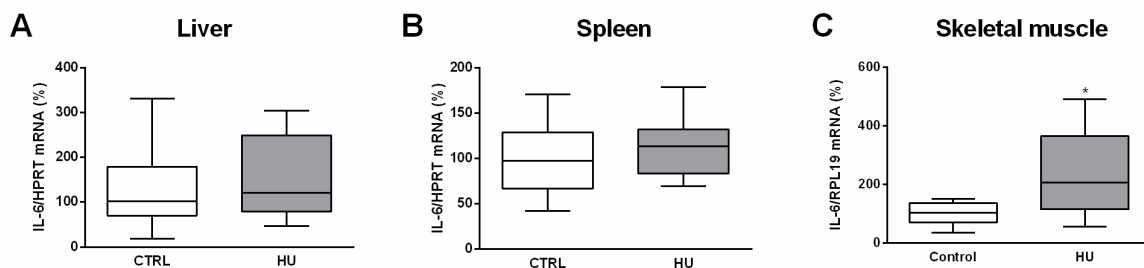
Figure 3. IL-6 mRNA increases in skeletal muscle of HU rats. A : IL-6 mRNA level in liver. B : IL-6 mRNA level in spleen. C : IL-6 mRNA level in gastrocnemius. Significance was checked using Mann-Whitney. *p<0.05
