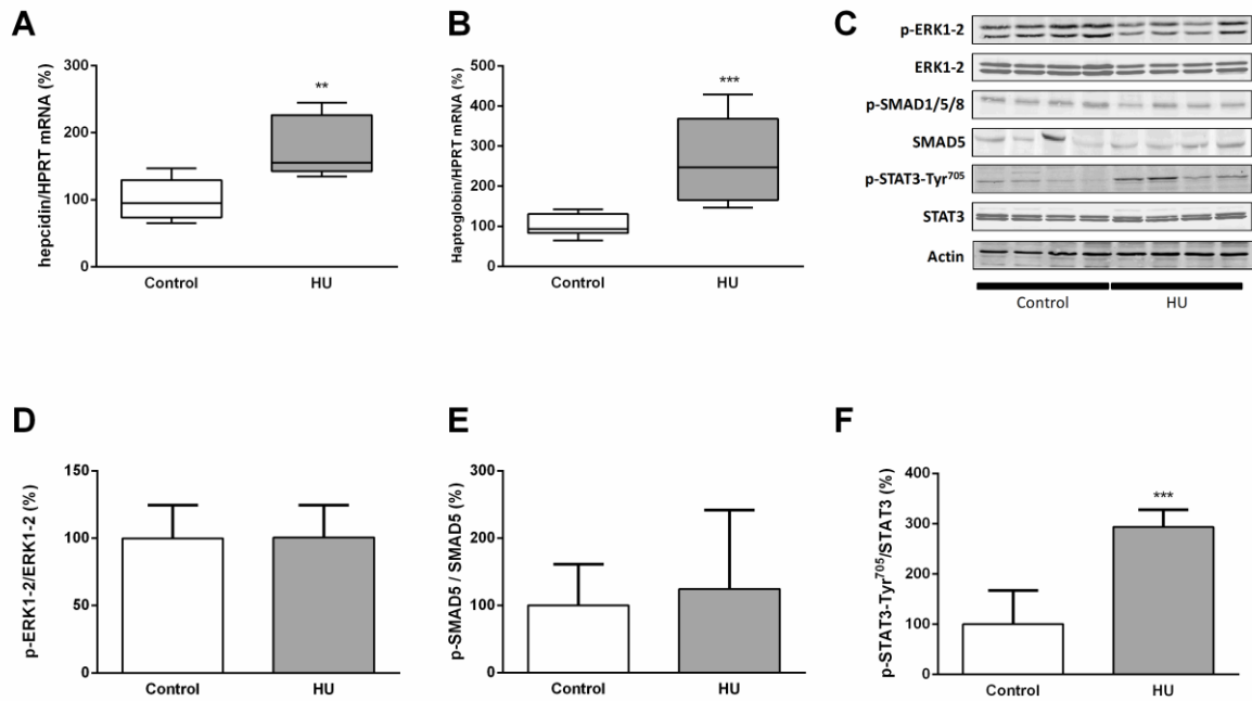
Figure 2. Hindlimb unloading induces hepatic hepcidin upregulation via the IL-6/STAT3 signaling pathway. A : Hepatic hepcidin mRNA level. B : hepatic haptoglobin mRNA level. C : representative blots of p-ERK1-2-Thr 202 /Tyr 204 , ERK1-2, p-SMAD1/5/8 Ser 463/465 , SMAD5, p-STAT3-Tyr 705 , STAT3 and actin. D : hepatic ERK1-2 activation. E : hepatic SMAD1/5/8 activation. F : hepatic STAT3 activation. Significance was checked using Mann-Whitney (A and B) or unpaired t-test (D, E and F). **p<0.01, ***p<0.001.
