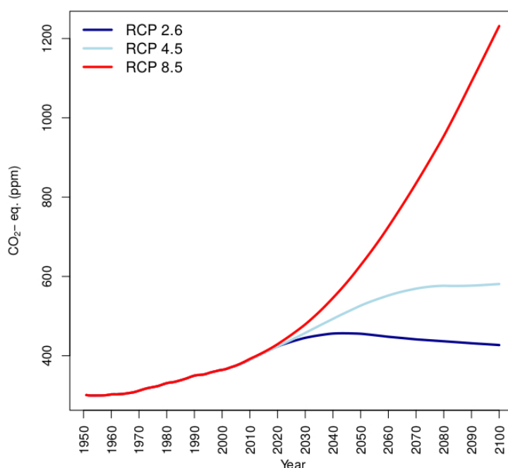
Figure 2. Evolution of the equivalent \text{CO}_2 for the three RCPs that describes the radiative forcing from greenhouse gases as used for the future simulations.
