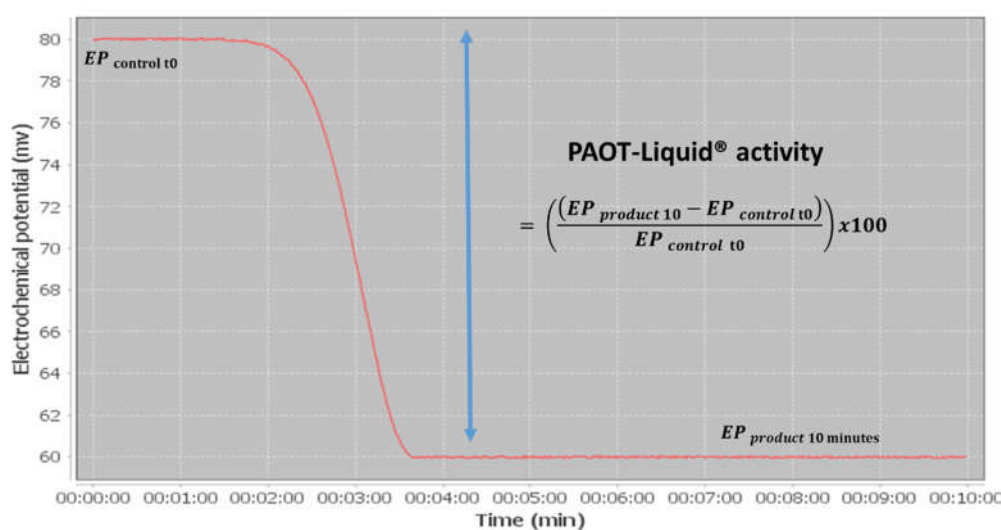
Figure 2. Kinetic curve of electrochemical potential changes during reaction of antioxidants or wines samples with the free radical mediator M^* .
