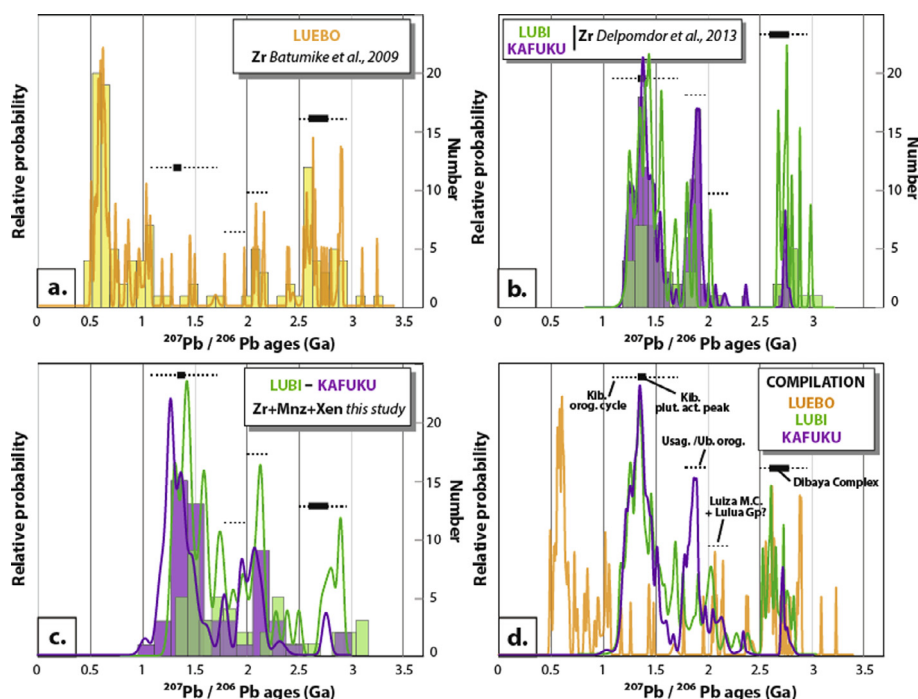
Fig. 9. ^{207}\text{Pb}/^{206}\text{Pb} apparent ages (Ga) on (a) zircons from the Luebo region (Batumike et al., 2009), (b) zircons from the Kafuku and Lubi drill cores (Delpomdor et al., 2013) and (c) xenotimes, monazites and zircons from the Kafuku and Lubi drill cores (this study). (d) Compilation of all ^{207}\text{Pb}/^{206}\text{Pb} apparent ages (Ga). Kibara plutonic activity peak, Kibara orogenic cycle, Usagara/Ubende orogeny, Luiza Metasedimentary Complex and Lulua Group.
