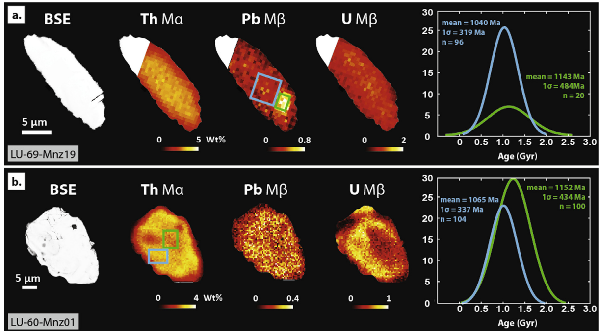
Fig. 6. Backscattered images and X-ray maps (Th M \alpha , Pb M \beta and U M \beta ) for two monazites from Lubi drill core and corresponding ages calculated (standard normal distribution of the pixel values from the green and blue areas), showing two distinct age domains, in core (in green) and in rims (in blue) respectively.
