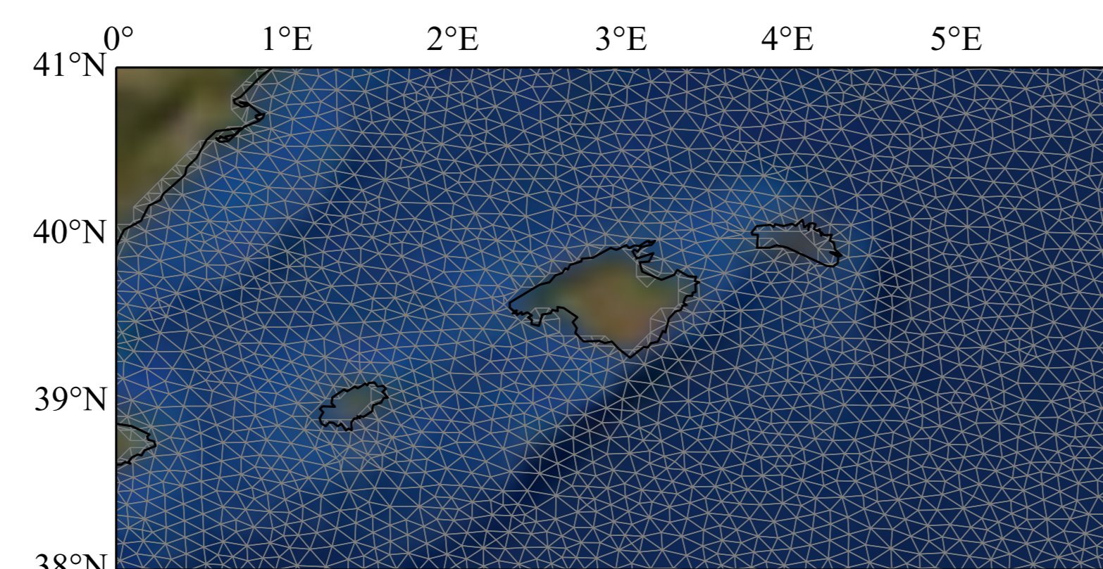
Figure 3: Finite-element mesh around the Balearic Islands. The typical size of the triangle is 1/6°.
