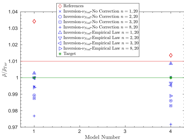
Figure 11. Inversion results for models 1 and 4 using patched model I from Sonoii et al. (2015) as target and varying the lowest n in the set of modes used for the inversion.
