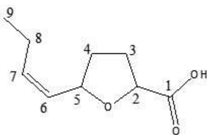
Figure 3: Structure of (6 Z )-2,5-Epoxyonon-6-enoic acid (2) used for DFT calculations.
