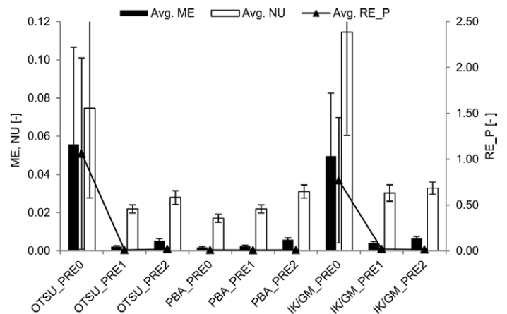
Fig. 8. Averaged misclassification error (ME), region non-uniformity (NU), and porosity relative error (RE_P) for all segmentation methods (OTSU, porosity-based [PBA], and adaptive indicator kriging + gradient masks [IK/GM]) and for all pre-segmentation noise reductions (PRE0, PRE1, and PRE2).
