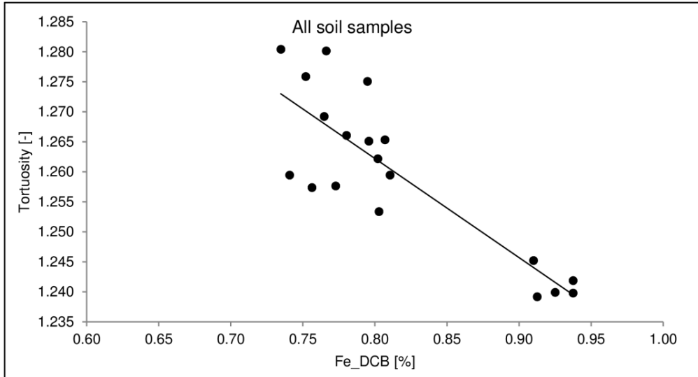
Figure 44. Tortuosity measured on the X-ray μCT images (τ) versus Fe extracted with DCB (Fe_DCB) for all soil samples.
