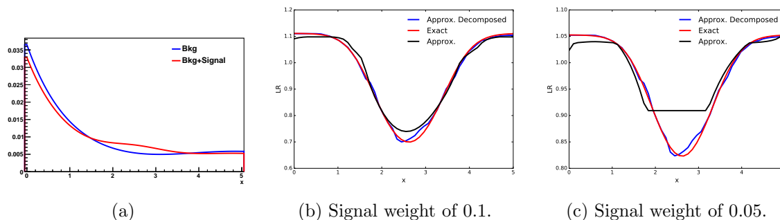
Figure 1: (1a) shows the mixture model distributions. (1b) and (1c) show a density ratio comparison for different values of the signal weight.
