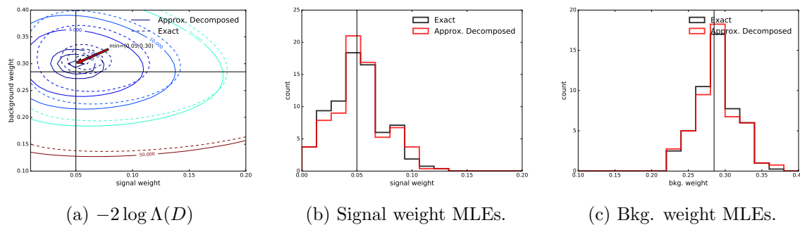
Figure 3: (3a) shows the values of -2 \log \Lambda(D) given the signal and one of the bkg. weights. (3b) and (3c) show histograms for maximum likelihood estimated values for the signal and background weights respectively.
