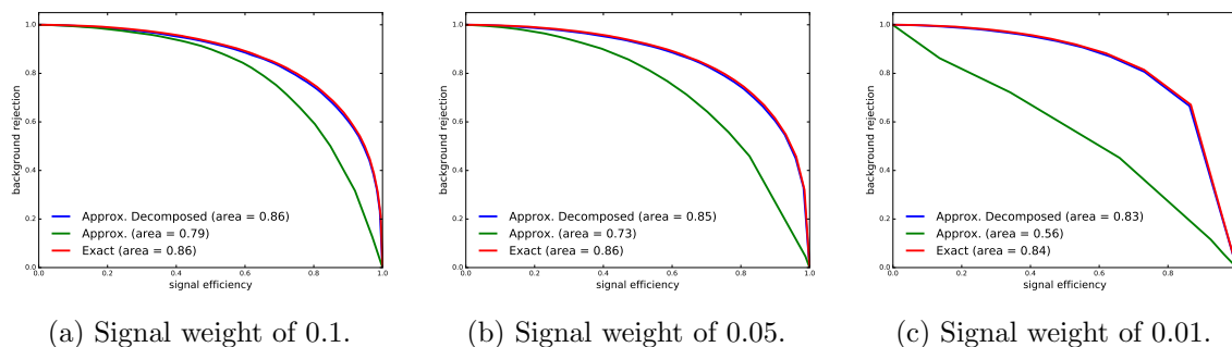
Figure 2: Background rejection versus signal efficiency curve comparison for different values of the signal weight.
