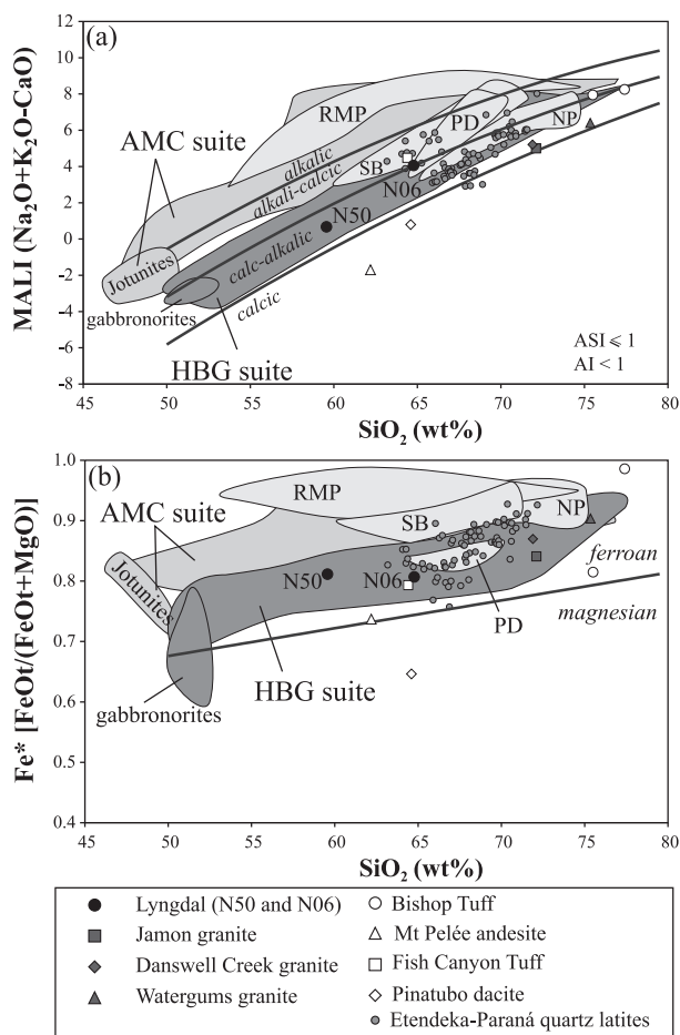
Fig. 1. (a) MALI index plotted as a function of wt % SiO 2 and (b) Fe* as a function of wt % SiO 2 for Proterozoic granitoids associated with massif anorthosites or similar affinities: granitoids from the Rogaland anorthositic complex [AMC suite (Anorthosite–Mangerite–Charnockite): Wilmart et al. (1989), Duchesne & Wilmart (1997)] and associated hornblende–biotite plutons of the HBG suite (Hornblende–Biotite Granitoids), Nain Province (NP: Emslie & Stirling, 1993), Laramie anorthositic complex [RMP (Red Mountain Pluton): Anderson et al. , 2003] and associated hornblende–biotite granitoids [SB (Sherman batholith): Frost et al. , 1999], Parker Dam [PD: Anderson & Bender (1989); the other plutons from that study are not plotted for clarity]. Mafic rocks associated with the HBG suite (gabbronorites: Demaiffe et al. , 1990; Bogaerts et al. , 2003a) and of the AMC suite are also plotted (jotunites: Vander Auwera et al. , 1998). Boundaries are from Frost et al. (2001). Data sources: Jamon granite from Dall’Agnol et al. (1999); Danswell Creek granite from Klimm et al. (2003); Watergums granite from Clemens et al. (1986); Bishop Tuff from Hildreth (1979), Etendeka–Paraná quartz latites from Garland et al. (1995) and Ewart et al. (1998); Fish Canyon Tuff from Johnson & Rutherford (1989b); Pinatubo dacite from Scaillet & Evans (1999); Mt. Pelée andesite from Martel et al. (1999).
