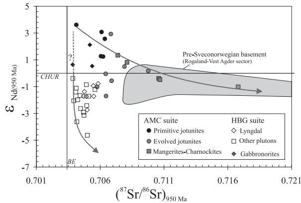
Fig. 10. \epsilon_{\text{Nd}}(950 \text{ Ma}) plotted as a function of the (^{87}\text{Sr}/^{86}\text{Sr})_{950 \text{ Ma}} for the HBG and AMC suites. The gabbronorites are also plotted. Data sources: Demaiffe et al. (1990); Bolle et al. (2003); Bogaerts et al. (2003a); Vander Auwera et al. (2003). The evolution from the jotunites to the charnockites (AMC suite) by crystallization and crustal contamination is well constrained (Duchesne & Wilmart, 1997; Vander Auwera et al. , 1998); the link between the jotunites–gabbronorites and the HBG suite is hypothetical (see text). BE: (^{87}\text{Sr}/^{86}\text{Sr})_{950 \text{ Ma}} for the Bulk-Earth calculated from present ratios of ^{87}\text{Sr}/^{86}\text{Sr} = 0.7047 and ^{87}\text{Rb}/^{86}\text{Sr} = 0.0850 ; \epsilon_{\text{Nd}} values are calculated relative to CHUR at 950 Ma with present ratios of ^{143}\text{Nd}/^{144}\text{Nd} = 0.512638 and ^{147}\text{Sm}/^{143}\text{Nd} = 0.1967 (Faure, 1986).
