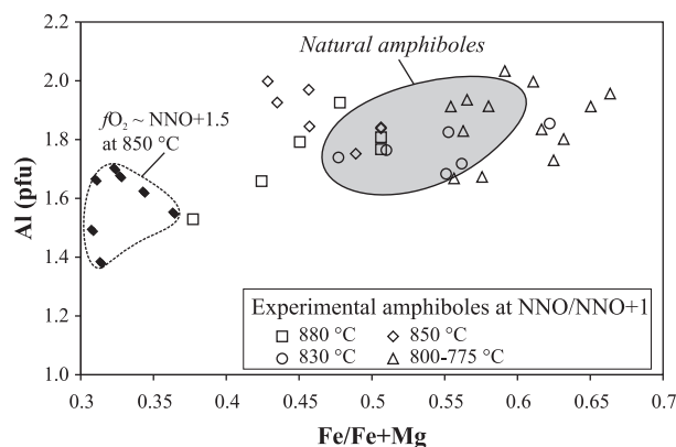
Fig. 6. Amphibole compositions: Al (a.p.f.u.) plotted against Fe/(Fe + Mg) ratios, illustrating the compositional variation of the experimental amphiboles with fO_2 and pressure. Natural amphibole compositions are depicted by the shaded area.
