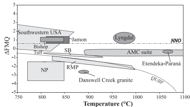
Fig. 9. \Delta FMQ [ \log fO_2(\text{sample}) - \log fO_2(\text{FMQ buffer}) ] vs temperature ( ^{\circ}\text{C} ), illustrating the diversity in fO_2 for metaluminous ferroan granitoids: Lyngdal (this study), AMC suite (Vander Auwera & Longhi, 1994; Duchesne & Wilmart, 1997), Jamon (Dall’Agnol et al. , 1999), Sherman batholith (SB: Frost et al. , 1999), Red Mountain Pluton (RMP: Anderson et al. , 2003), plutons from the Nain Province (NP: Emslie & Stirling, 1993), plutons from the Southwestern USA (Anderson & Bender, 1989), Danswell Creek granite (King et al. , 2001; Klimm et al. , 2003). T – fO_2 conditions estimated for the Bishop Tuff (Frost & Lindsley, 1992) and the Etendeka–Paraná quartz latites to rhyolites (Bellieni et al. , 1986) are also plotted. The QUIL curve refers to the Quartz–Ulvöspinel–Ilmenite–Fayalite equilibrium after Andersen et al. (1993).
