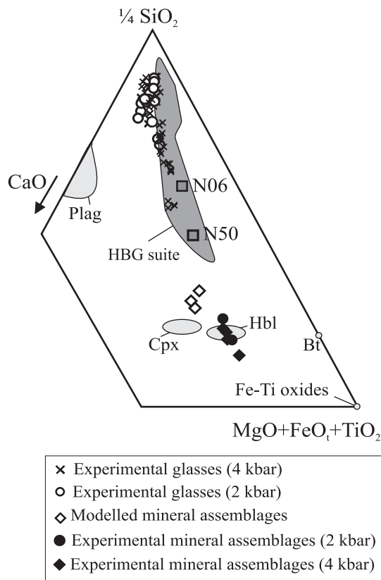
Fig. 7. 1/4\text{SiO}_2\text{-CaO-(MgO + FeO}_t + \text{TiO}_2) diagram (molar proportions) comparing experimental glasses with natural rocks from the HBG suite [data from Bogaerts et al. (2003a) and Vander Auwera et al. (2003); N06 and N50 correspond to the starting products]. The modelled mineral assemblages are obtained based on major element modelling by the least-squares method on natural rocks (Bogaerts et al. , 2003a). The modal proportions of representative experimental mineral assemblages are given in Table 11. Plag, plagioclase; Cpx, clinopyroxene; Hbl, amphibole; Bt, biotite.
