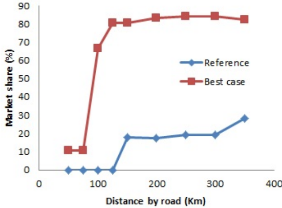
Fig. 3. Effect of all-road/trucking market size on the intermodal market share.
