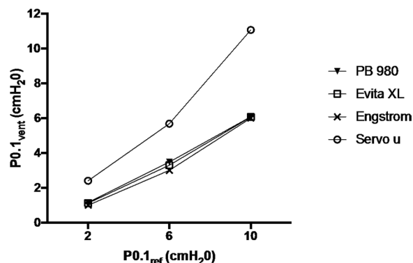
Fig. 1 Analysis of ventilator measurements
