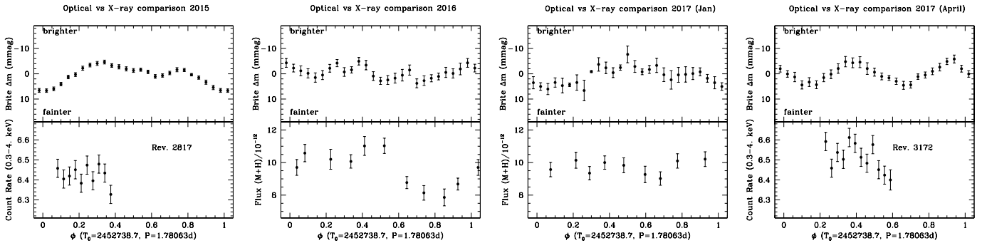
Fig. 10. Same as Figure 9 but using epochally averaged BRITE light curves valid for the date of the X-ray observations (cycles associated with “Part V” data for April 2015, “Part VI” for Dec 2016, “Part VII” for Jan 2017, and “Part IX” for April 2017, for details see Ramiamanantsoa et al. 2017a, submitted). The ephemerides are those adopted by Ramiamanantsoa et al. (2017a, submitted).
