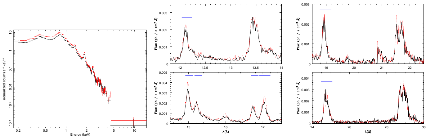
Fig. 6. Comparison of the pn (left) and RGS (middle and right) spectra observed at minimum brightness (first part of Rev. 1814; solid black line) and maximum brightness (first part of Rev. 2183; dotted red line). Blue segments above lines of RGS spectra indicate the intervals chosen for the moment calculations.
