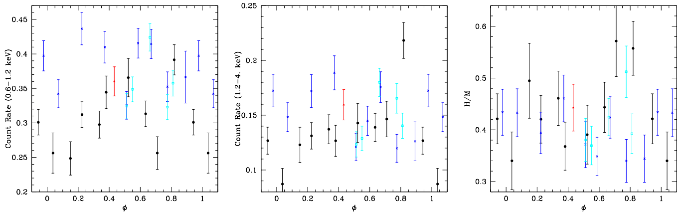
Fig. 4. Same as Figure 1 but for Swift data; those from Oct. 2016, Dec. 2016, Jan. 2017, and April 2017 are shown as red triangles, black dots, blue crosses, and cyan squares, respectively.
