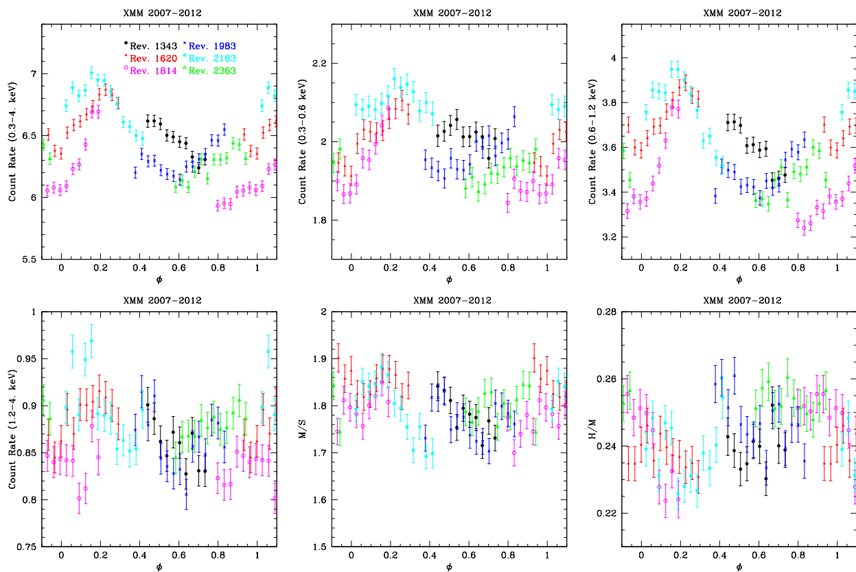
Fig. 2. Same as Figure 1 but for XMM-Newton data from 2007–2012.
