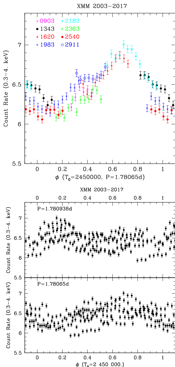
Fig. 8. Subgroup of XMM-Newton light curves can be phased with a period of 1.78065 d to form a relatively coherent behaviour (top), but considering all available light curves only lead to scatter plots, whatever the value of the 1.78 d period considered (bottom).
