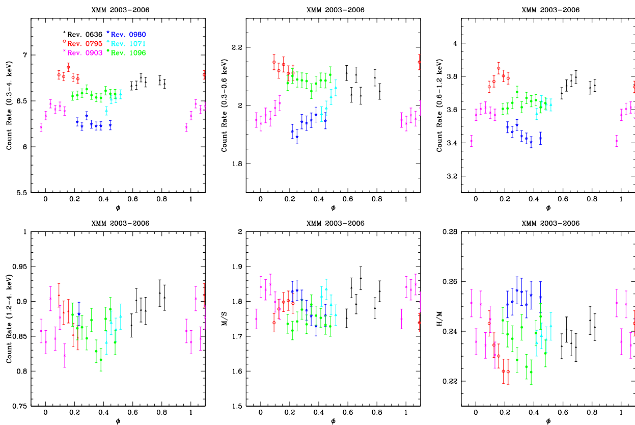
Fig. 1. Count rates in several energy bands of \zeta Pup, and associated hardness ratios for XMM-Newton data from 2003–2006. The phases were calculated using P = 1.780938 d and T_0 = 2\,450\,000 (Howarth & Stevens 2014). To facilitate the comparisons, the ratio between upper and lower limits of the y-axes are all equal.
