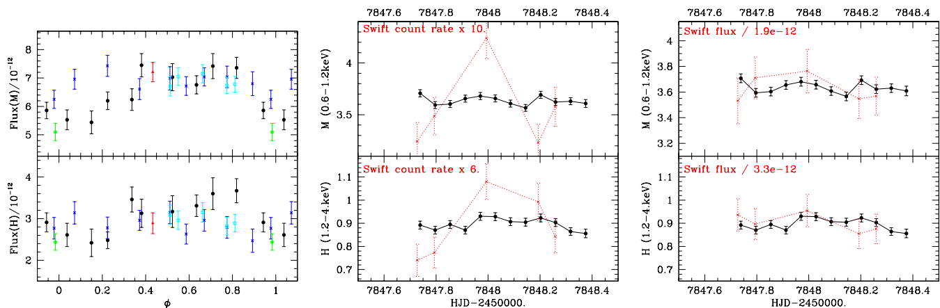
Fig. 7. Left: Same as Figure 4 but for the fluxes (Table 4). The green stars correspond to data from February 2013. Middle and right: Comparison between the XMM-Newton light curve of April 2017 (Rev. 3172, black dots and solid lines) and the (arbitrarily scaled) simultaneous Swift light curve (red crosses and dotted lines) derived from count rates (middle) or fluxes (right).
