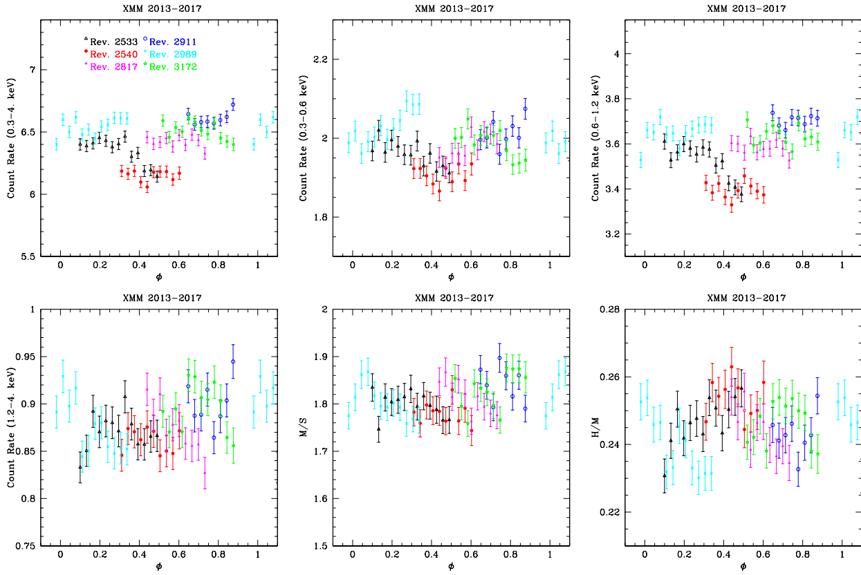
Fig. 3. Same as Figure 1 but for XMM-Newton data from 2013–2017.
