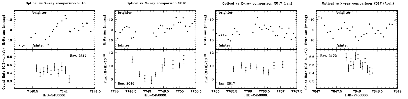
Fig. 9. Comparison of the X-ray light curves with the simultaneous BRITE photometry in April 2015 (combined light curve from the two BRITE filters, for details see Ramiamanantsoa et al. 2017a, submitted), and December 2016–April 2017 (only one satellite, BRITE -Lem, in the blue filter, see Ramiamanantsoa et al. 2017b, in prep). For Swift , fluxes from the spectral fits (Table 4) are used since they are more reliable.
