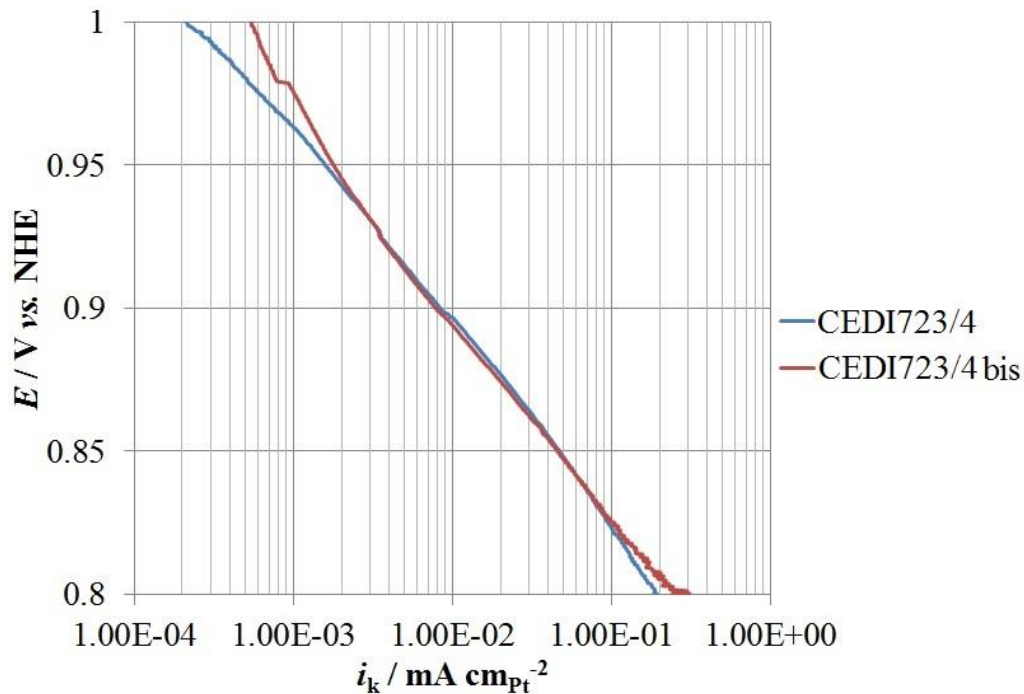
Figure SI.2 Tafel plot of the CEDI723/4 catalyst measured twice (reproducibility measurement).
