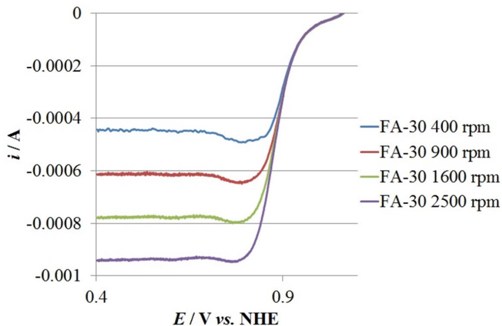
Figure SI.1 ORR measurements performed at four different rotating speeds of the electrode (400, 900, 1,600, and 2,500 rpm) for the FA-30 catalyst.
