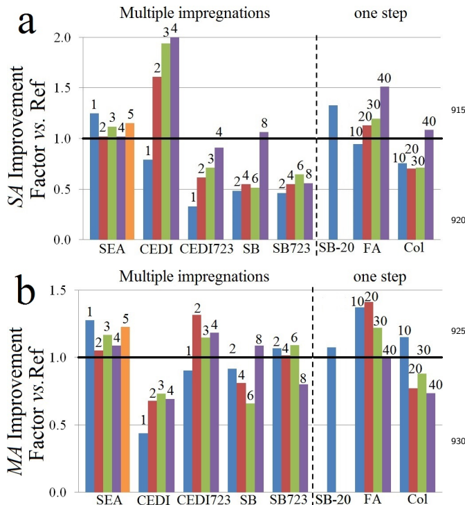
Figure 5: SA (a) and MA (b) improvement factor vs. Ref. The horizontal black line represents improvement factor of 1, i.e. the position of the reference (commercial catalyst). The number upon each bar represents the number of impregnations the catalyst underwent (in the case of multiple impregnations methods) or the targeted loading (in the case of one-step methods).
