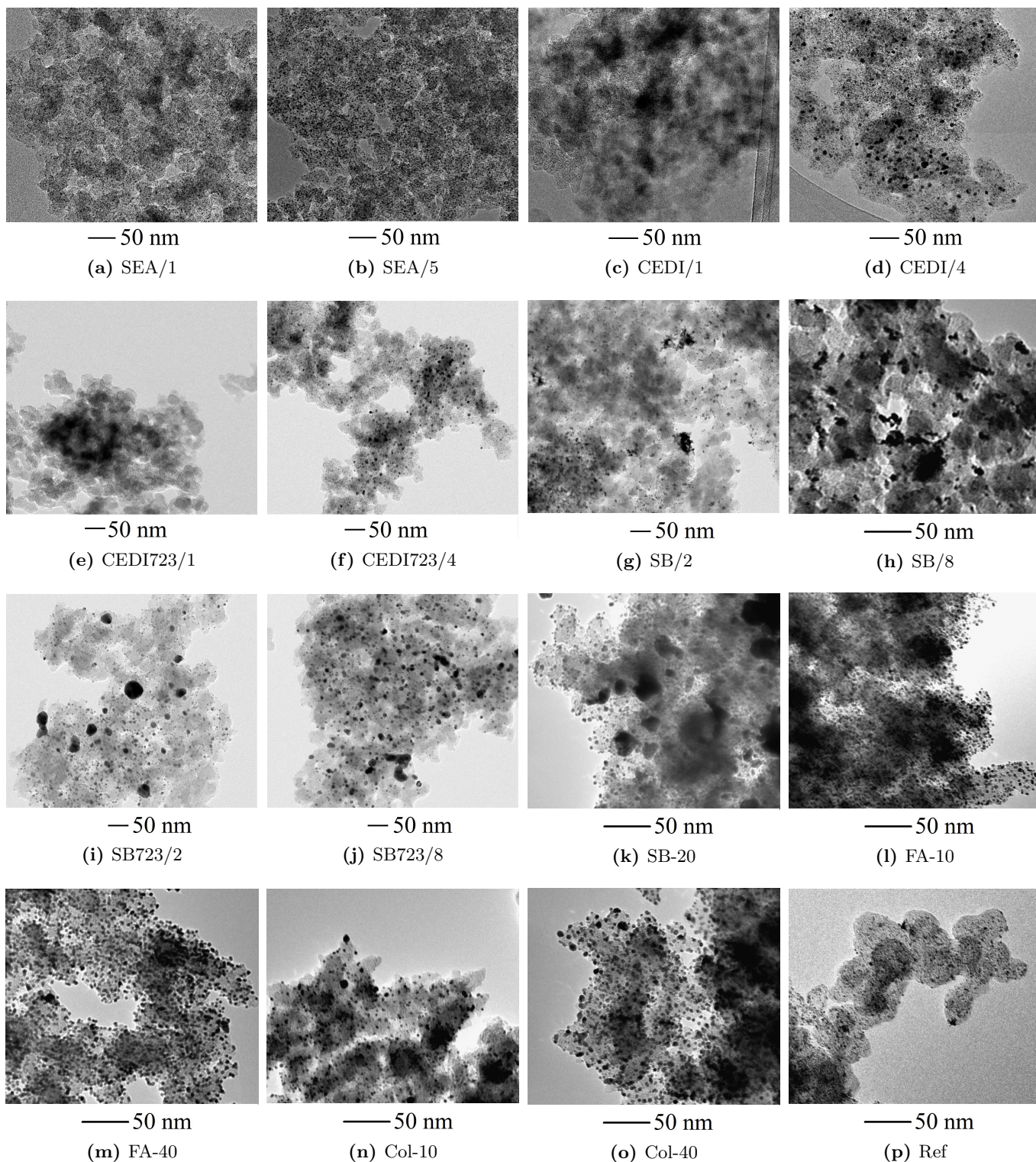
Figure 1: TEM micrographs of the catalysts with the lowest and the highest loading for each synthesis and the commercial catalyst: SEA/1 (a), SEA/5 (b), CEDI/1 (c), CEDI/4 (d), CEDI723/1 (e), CEDI723/4 (f), SB/2 (g), SB/8 (h), SB723/2 (i), SB723/8 (j), SB-20 (k), FA-10 (l), FA-40 (m), Col-10 (n), Col-40 (o), and Ref (p).
