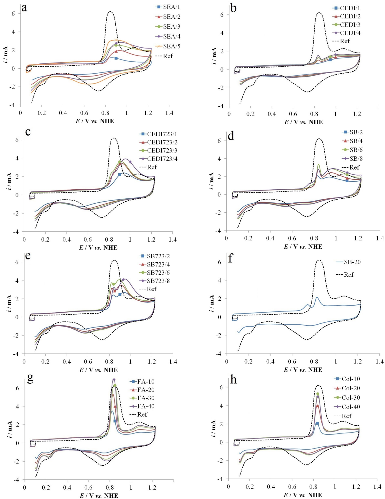
Figure 4: CO electrooxidation voltammograms of all the catalysts in 1 M \text{H}_2\text{SO}_4 at a sweep rate of 20 \text{ mV s}^{-1} at room temperature: SEA/1 to SEA/5 (a); CEDI/1 to CEDI/4 (b); CEDI723/1 to CEDI723/4 (c); SB/2 to SB/8 (d); SB723/2 to SB723/8 (e); SB-20 (f); FA-10 to FA-40 (g); Col-10 to Col-40 (h). The voltammogram of the Ref sample (dotted line) is reported in each case for comparison.
