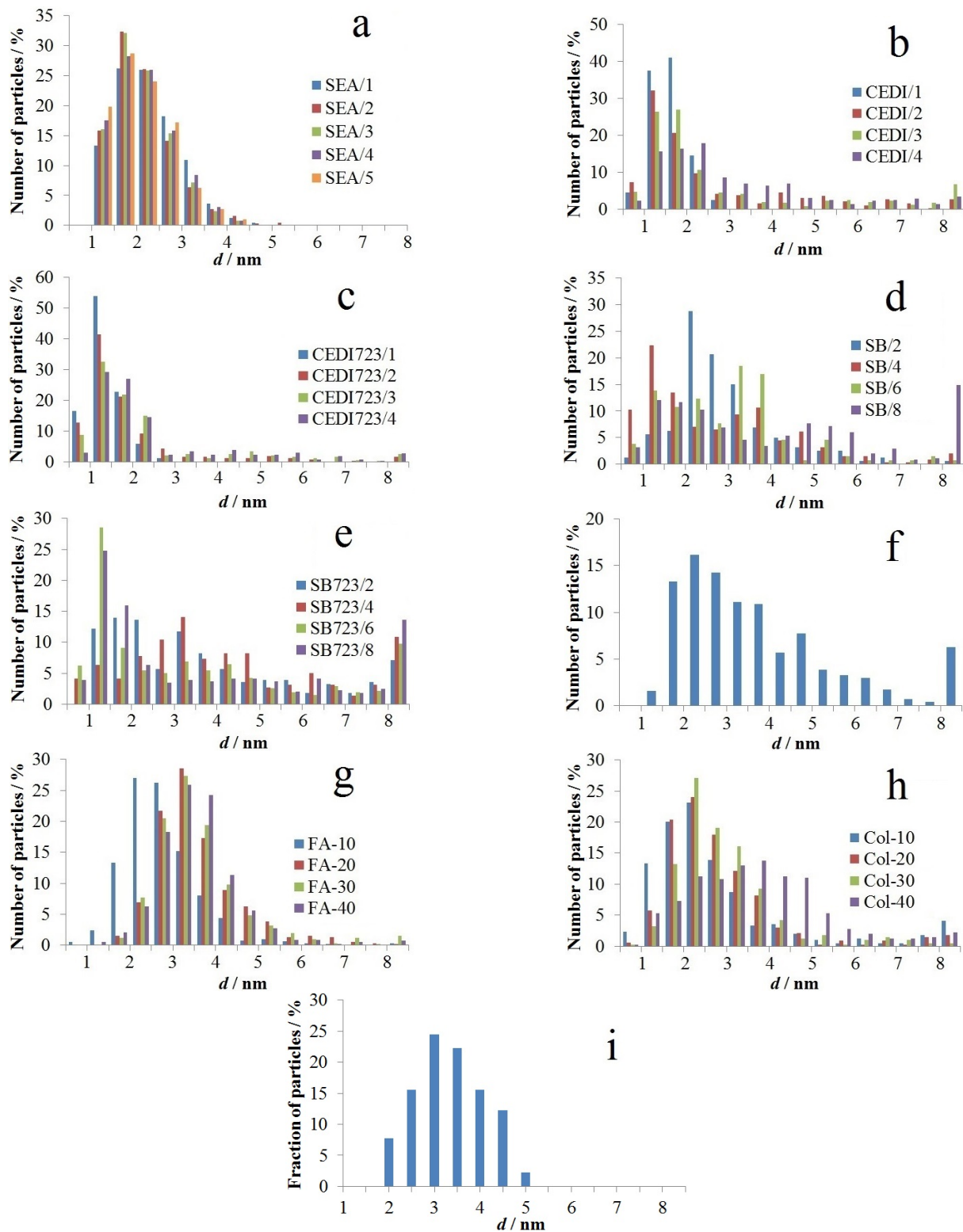
Figure 2: Pt particle size distribution histograms of all the catalysts obtained by image analysis: SEA/1 to SEA/5 (a); CEDI/1 to CEDI/4 (b); CEDI723/1 to CEDI723/4 (c); SB/2 to SB/8 (d); SB723/2 to SB723/8 (e); SB-20 (f); FA-10 to FA-40 (g); Col-10 to Col-40 (h); and of the reference catalyst, Ref (i). The last category of the histograms represents the fraction of Pt particles with diameter higher than 8 nm.
