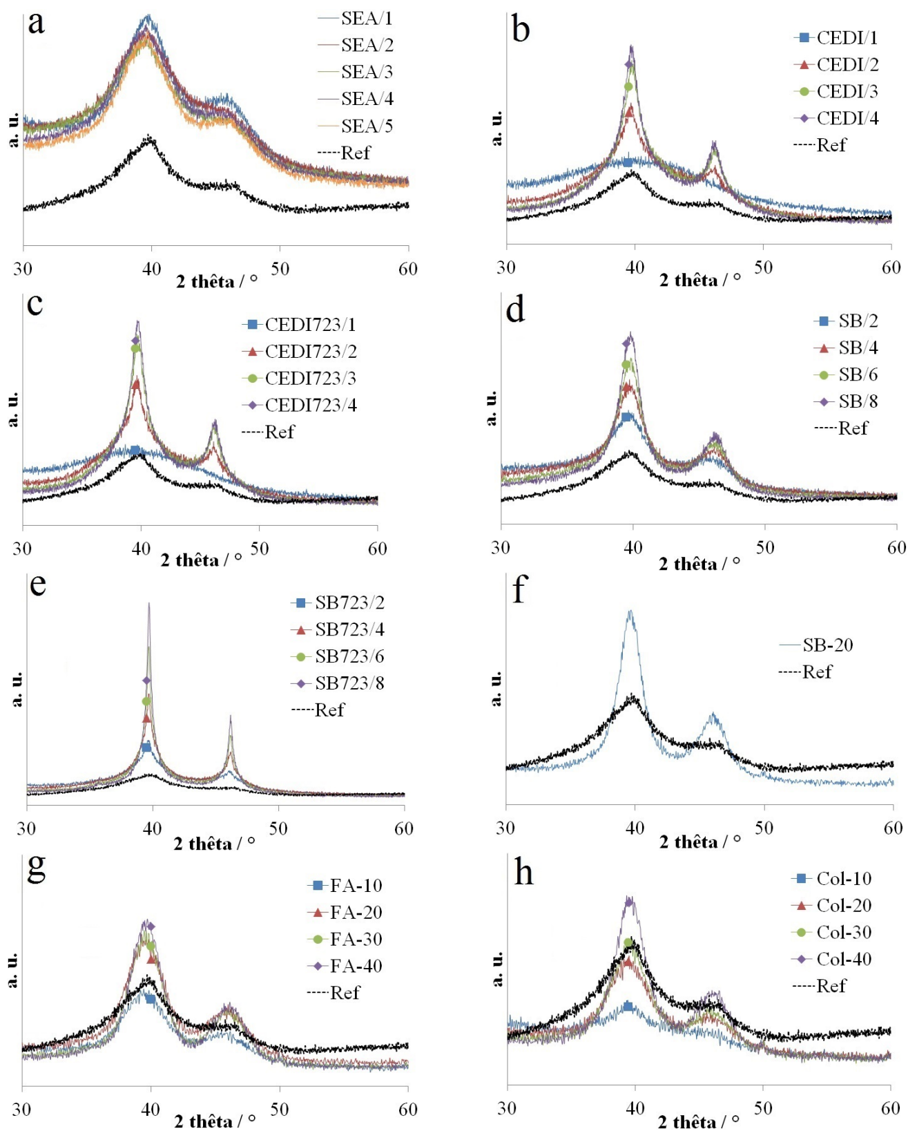
Figure 3: XRD diffractograms of all the catalysts: SEA/1 to SEA/5 (a); CEDI/1 to CEDI/4 (b); CEDI723/1 to CEDI723/4 (c); SB/2 to SB/8 (d); SB723/2 to SB723/8 (e); SB-20 (f); FA-10 to FA-40 (g); Col-10 to Col-40 (h). The Ref diffractogram (dotted black line) serves as a basis for comparison.
