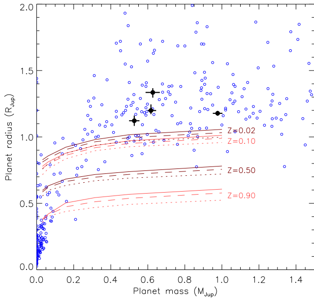
Figure 11. As Fig. 10 but with different theoretical predictions. The lines show the predicted planet radii of gas-giants from Baraffe et al. (2008, their table 4) for four different heavy-element mass fractions Z , labelled on the plot. The unbroken lines show predictions for a planet of age 0.5 Gyr, the dashed lines for an age of 1 Gyr and the dotted lines for an age of 5 Gyr. The lines are colour-coded for clarity.
