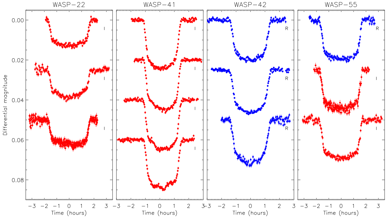
Figure 1. DFOSC light curves presented in this work, in the order they are given in Table 1. Times are given relative to the midpoint of each transit, and the filter used is indicated. Blue and red filled circles represent observations through the Bessell R and I filters, respectively.
