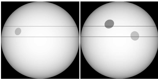
Figure 7. Visualisations of the surface of WASP-41 A at the times of the third (left) and fourth (right) transits we observed with DFOSC, produced by PRISM. The boundaries of the path of the planet are shown with black lines and the spots are shown with their measured locations, sizes and contrasts.
