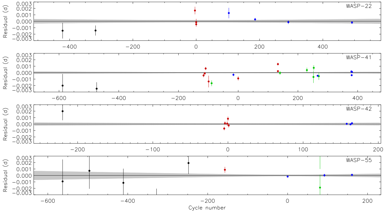
Figure 9. Plot of the residuals of the timings of mid-transit versus a linear ephemeris. The results from this work are shown in blue and from amateur observers in green. Our reanalysis of published data are shown in black for WASP-South observations and in red for other sources. The grey-shaded regions show the 1\sigma uncertainty in the ephemeris as a function of cycle number.
