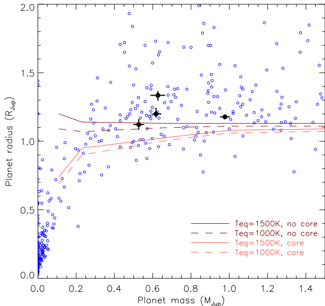
Figure 10. Plot of planet radii versus their masses. WASP-22 b, WASP-41 b, WASP-42 b and WASP-55 b are indicated using black filled circles. The overall population of planets is shown using blue open circles without errorbars, using data taken from TEPcat on 2015/11/09. The lines show the predicted planet radii of gas-giants from Bodenheimer et al. (2003, their table 1) for two different equilibrium temperatures (1000 K and 1500 K) which bracket the four planets, and for with and without a solid 20 M_{\oplus} core (see key).
