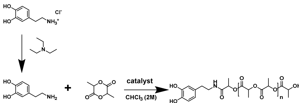
Scheme 1. Ring-opening polymerization for dopamine end-capped polylactide (PLLA).
