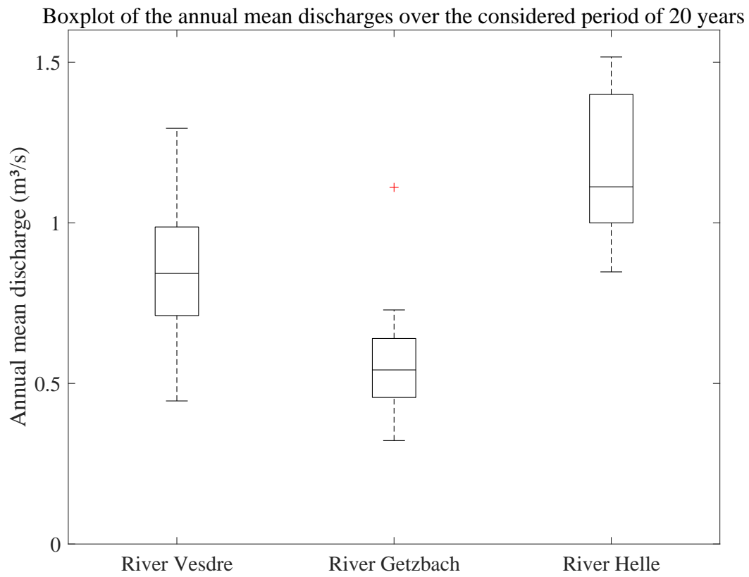
Figure A1 Boxplot of the annual mean discharges in the three rivers upstream of the reservoir over the considered period of 20 years (Vesdre, Getzbach and Helle).
