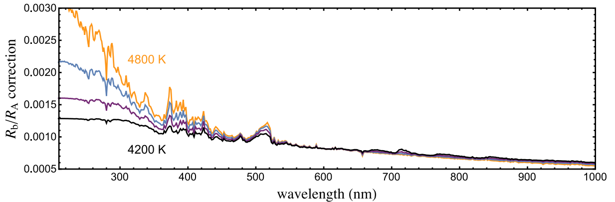
Figure 11. The effect of unocculted star-spots on the transmission spectrum of WASP-52 b, considering a 1% flux drop at 600 nm. A stellar temperature of T_{\text{eff}} = 5000 K was adopted. The star-spot coverage was modelled using a grid of stellar atmospheric models at different temperature ranging from 4800K (yellow line) to 4200K (black line), in steps of 200 K.
