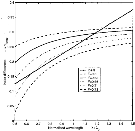
Figure 3. Search of tangency between linear ideal birefringence and effective ones.
