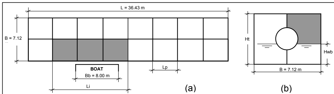
Figure 2: Example for Damaged Floating Tanks
