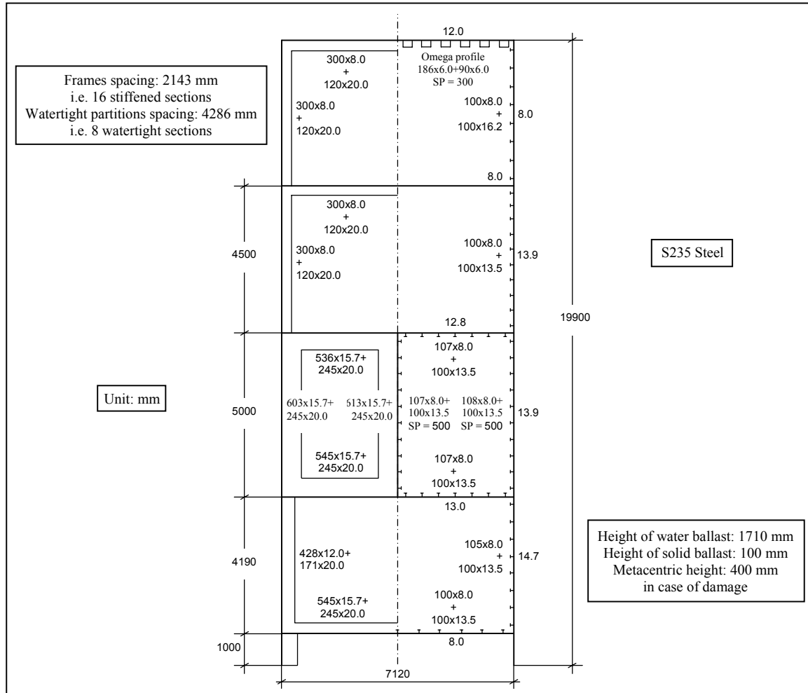
Figure 6: Optimized Van Cauwelaert Lock Gate
