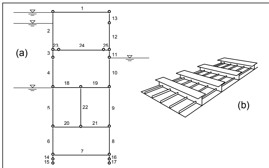
Figure 3: LBR-5 Modelling (a) Mesh Model of the Van Cauwelaert Lock Gate (b) Stiffened Panel Element
