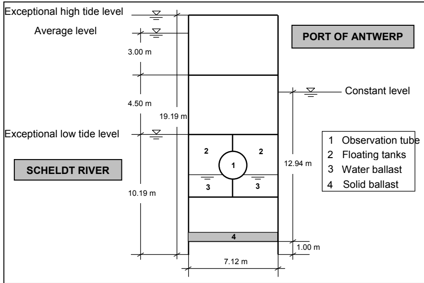
Figure 1: Cross-Section of the Van Cauwelaert Lock Gate
