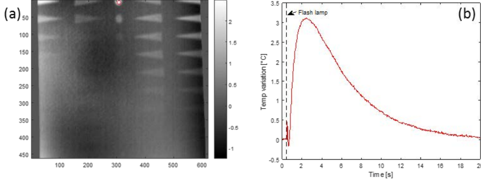
Figure 5. Thermography processing and result. (a) One thermogram of the full temporal sequence after processing; the red circle indicates the defect location. (b) Net and corrected temporal evolution of temperature at defect.
