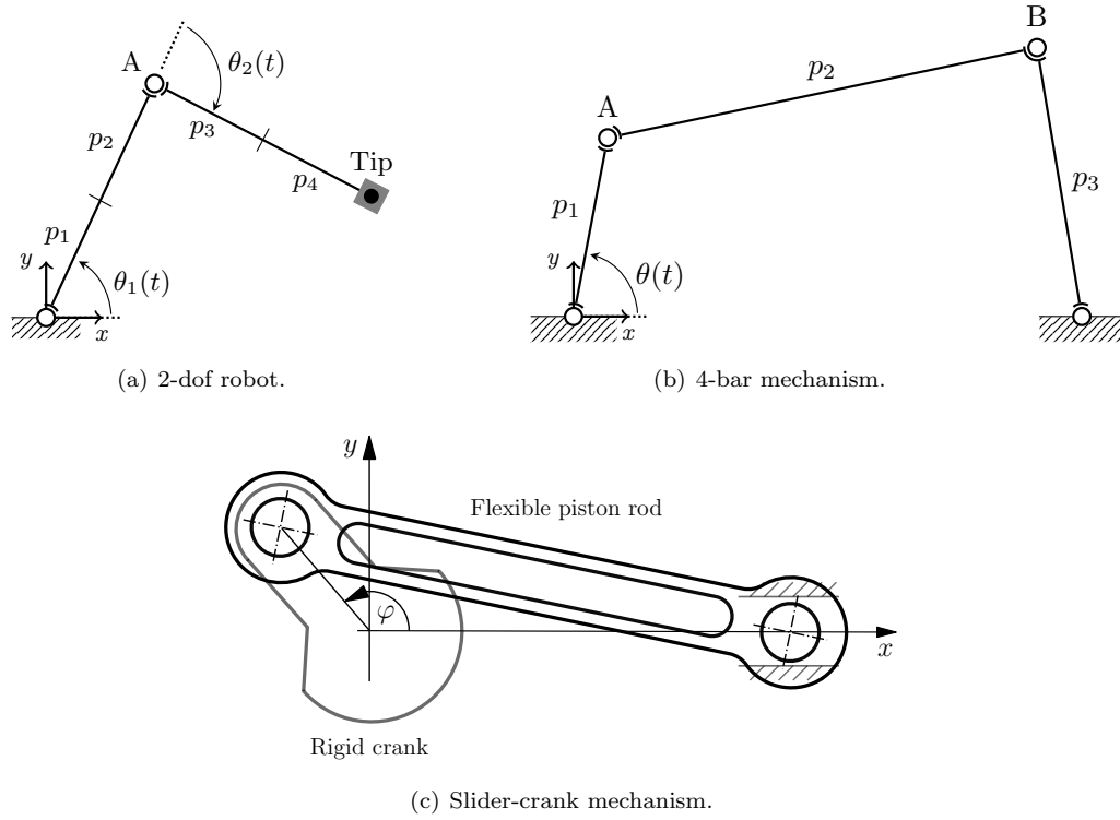
Figure 12: Some standard MBS design problems.
