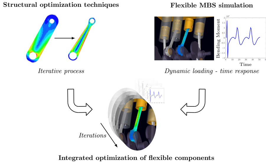
Figure 1: System-based approach for the design of flexible mechanisms.
