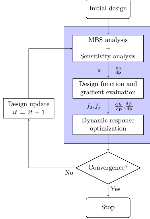
Figure 7: Fully coupled method framework.
