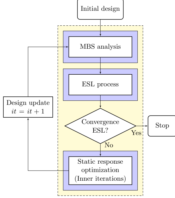
Figure 10: Weakly coupled method framework.
