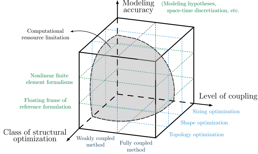
Figure 2: 3-dimensional space of the design complexity in structural optimization of flexible MBS. The classification of the methods adopted in the figure aims to be general but exceptions may exist.
