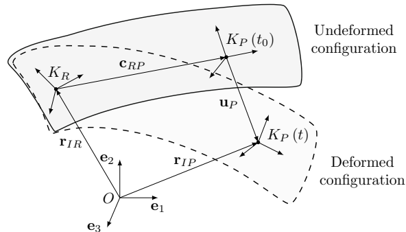
Figure 4: Kinematics of a flexible body using the floating frame of reference approach.
