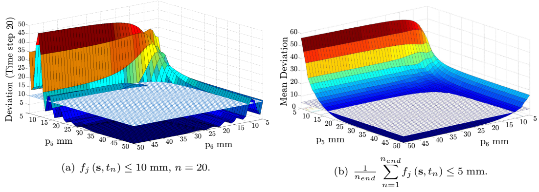
Figure 8: Design space representation for a local formulation at time step n = 20 (a) and for a global formulation (b), from [138].
