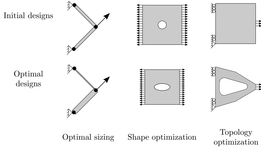
Figure 5: Structural optimization parameterizations.
