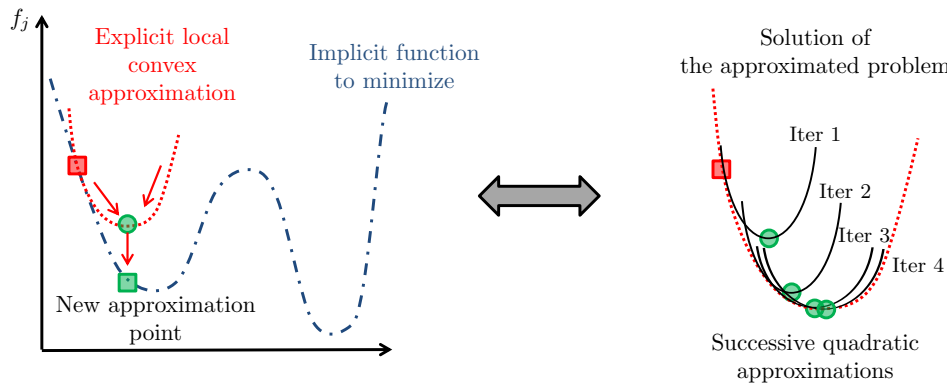
Figure 9: Sequential convex programming.
