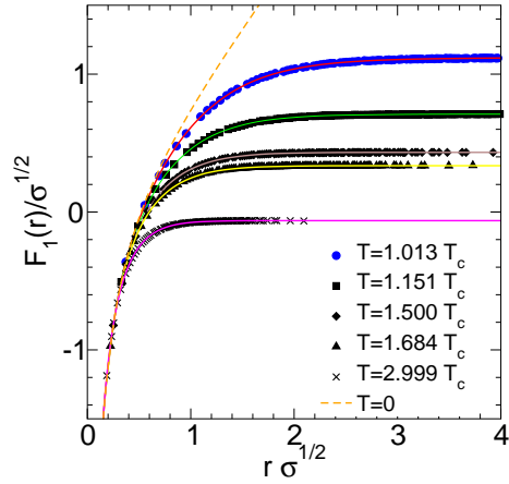
FIGURE 6. The colour singlet Q\bar{Q} free energy F(r, T) vs. r at different T [108, 109].
