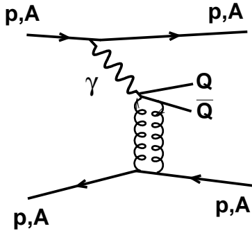
FIGURE 4. Schematic diagram for exclusive diffractive quarkonium photoproduction in \gamma A, p collisions.
