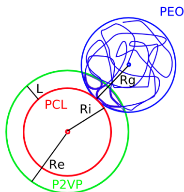
Figure 2 The core of PCL is spherical, hydrophobic. The thickness of the peel is L and the PEO chains are supposed gaussians.
