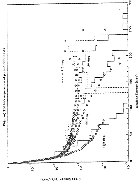
Fig. 7 : Comparison of neutron double differential cross-section data (ref. 14) with the predictions of the Liège INC model (from ref. 84). Only the cascade component is shown.
