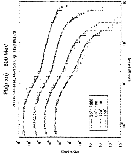
Fig. 6 : Neutron double differential cross-section data (ref. 66) compared with the INC calculations of ref. 64.
