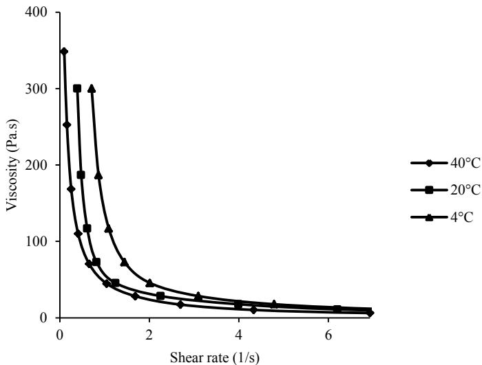
Figure 3 Effect of temperature on viscosity curves of pesto sample with 0.8 % of wax. (▲) sample stored at 4°C; (■) sample stored at 20°C; (●) sample stored at 40°C.
