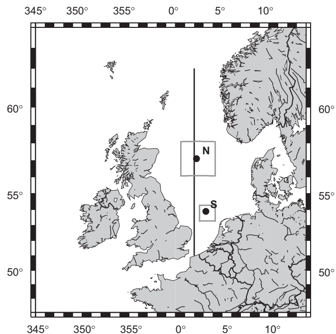
Fig. 2. The model domain including the North Sea, showing the section along 2° E (cf. Fig. 1), location N (57.1° N, 2.25° E) and location S (53.9° N, 3.25° E). The gray boxes show the areas used for spatial averages of DIC and \Delta pCO_2 in Figs. 5 and 6.
