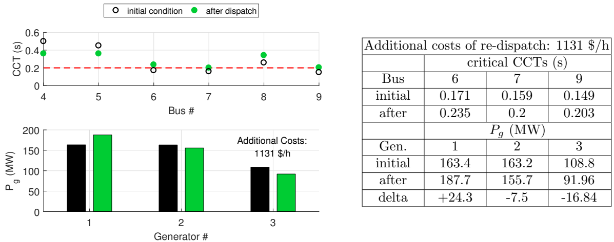
Figure 7: CCTs and active power setpoints for the initial condition and after the successful re-dispatch
