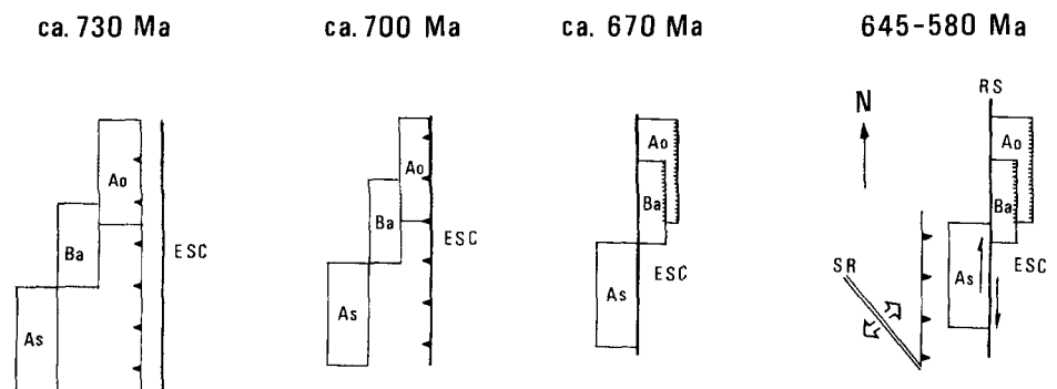
Figure 2. Plan views of relative movements of terranes of Air region during Pan-African orogeny. Lines with arrowheads indicate subduction trenches; ESC is East Saharan craton; Ao is Aouzegueur; Ba is Barghot; As is Assodé-Issalane; RS is Raghane shear zone; SR is spreading ridge. For dimension of terranes, see Figure 3. At ca. 670 Ma, thrusting of Aouzegueur and Barghot onto East Saharan craton ended while Assodé collided with craton; lithospheric thickening was followed by continental lithospheric mantle delamination. Between 645 and 580 Ma, Assodé moved north ~1000 km along Raghane shear zone, and there was abundant calc-alkaline magmatism in Assodé. For more details, see Liégeois et al. (1994).
