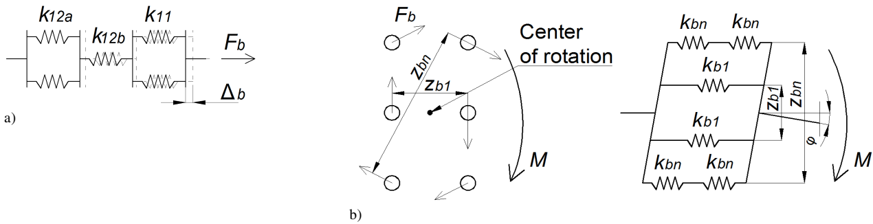
Fig. 4. a) Extensional spring system for one bolt b) Rotational spring for a bolt group
