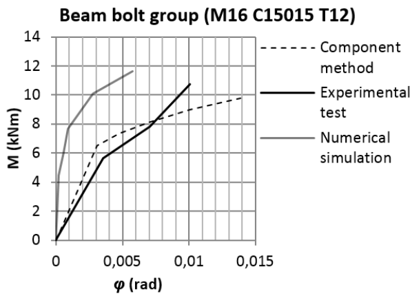
Fig. 11. M - \varphi curves of the beam bolt group of the specimens: a) M12 C15015 T12; b) M12 C15015 T12; c) M16 C15015 T12
