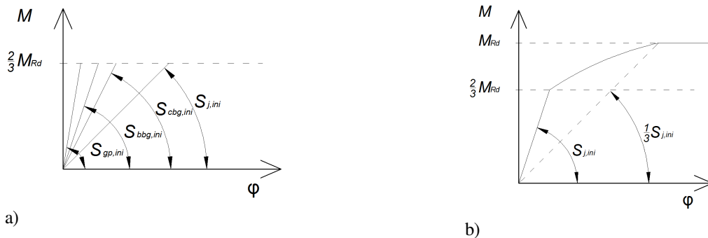
Fig. 6. a) Initial rotational stiffness of springs and joint b) M - \varphi relationship of joint
