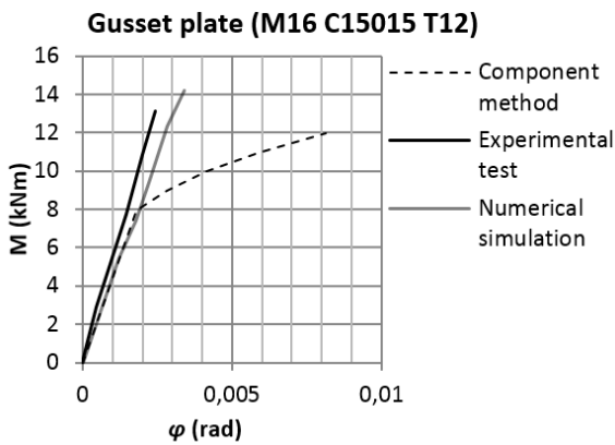
Fig. 13. M - \phi curves of the gusset plate of the specimens: a) M12 C15015 T12; b) M12 C15015 T12; c) M16 C15015 T12
