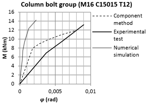
Fig. 12. M - \phi curves of the column bolt group of the specimens: a) M12 C15015 T12; b) M12 C15015 T12; c) M16 C15015 T12
