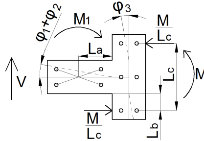
Fig. 5. The scheme for the rotation calculation of the gusset plate
