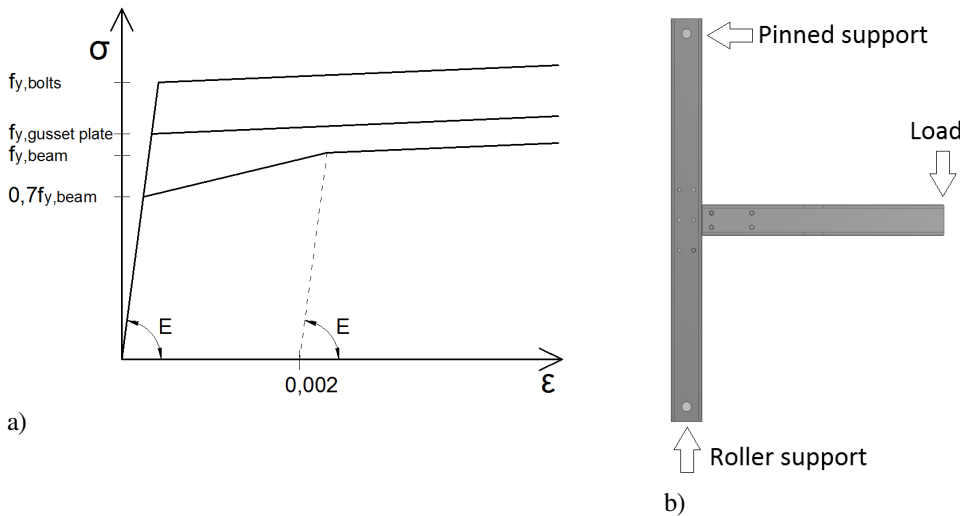
Fig. 10. a) Stress – strain relationships; b) Numerical model
