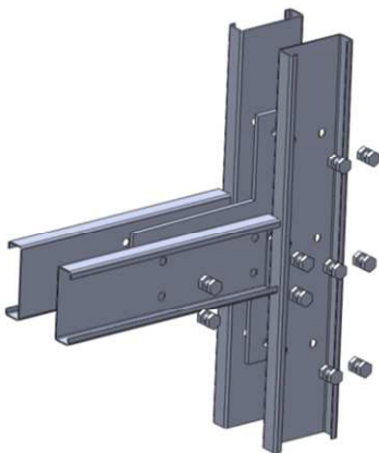
Fig. 1. The exploded view of the joint under analysis
