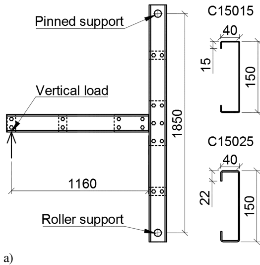
Fig. 7. a) Geometrical properties of the specimens b) 1, 2 – lateral restraints of the beam and the column, 3 – roller support with vertical moving direction, 4 – pinned support
