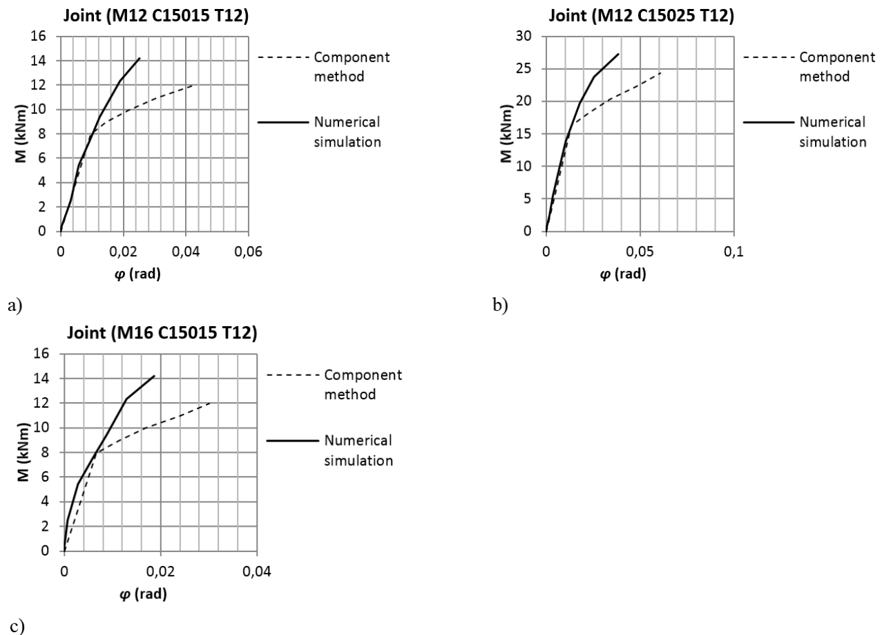
Fig. 14. M - \varphi curves of joints: a) M12 C15015 T12; b) M12 C15015 T12; c) M16 C15015 T12
