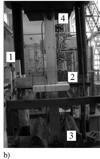
Fig. 7. a) Geometrical properties of the specimens b) 1, 2 – lateral restraints of the beam and the column, 3 – roller support with vertical moving direction, 4 – pinned support
