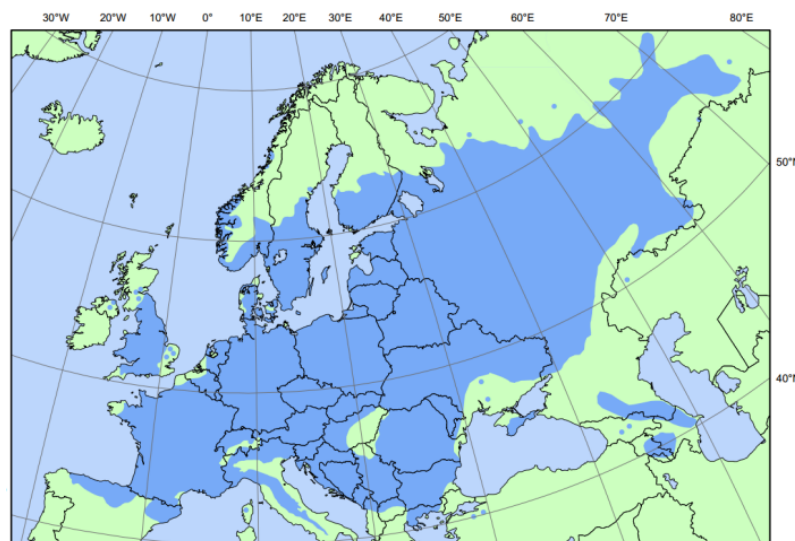
Figure 2. European distribution of T. cordata [91].
