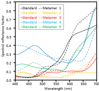
Fig. 3 - Spectral reflectances R(\lambda) of five metameric pairs used in the evaluation of D65 simulators in the visible range.
