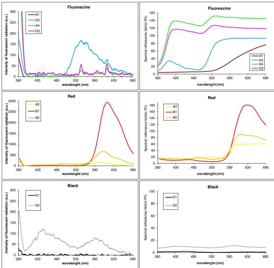
Fig. 4 – Intensity of fluorescence (left) and spectral reflectance factor (right) of the realized samples.
