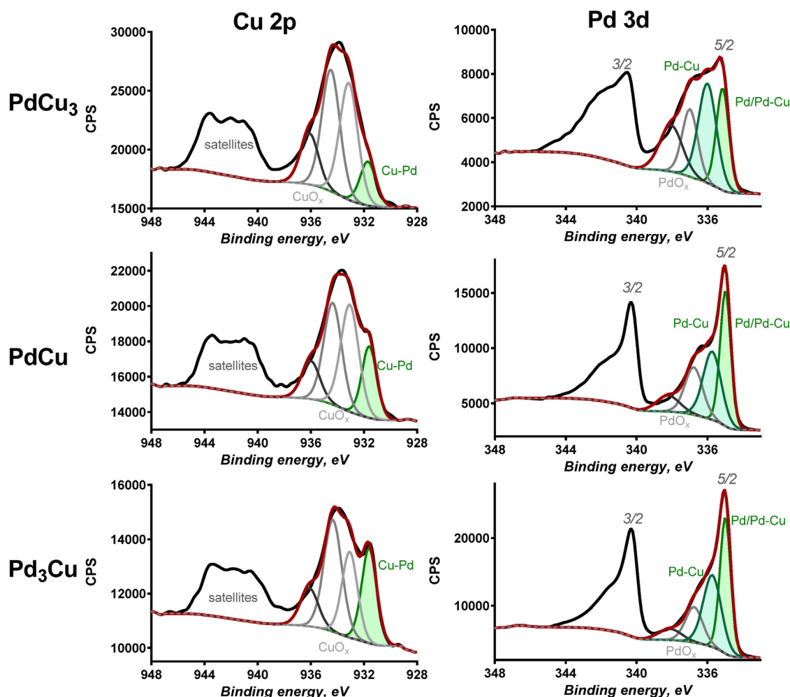
Fig. 3. High resolution XPS spectra of PdCu 3 , PdCu and Pd 3 Cu electrocatalyst.
