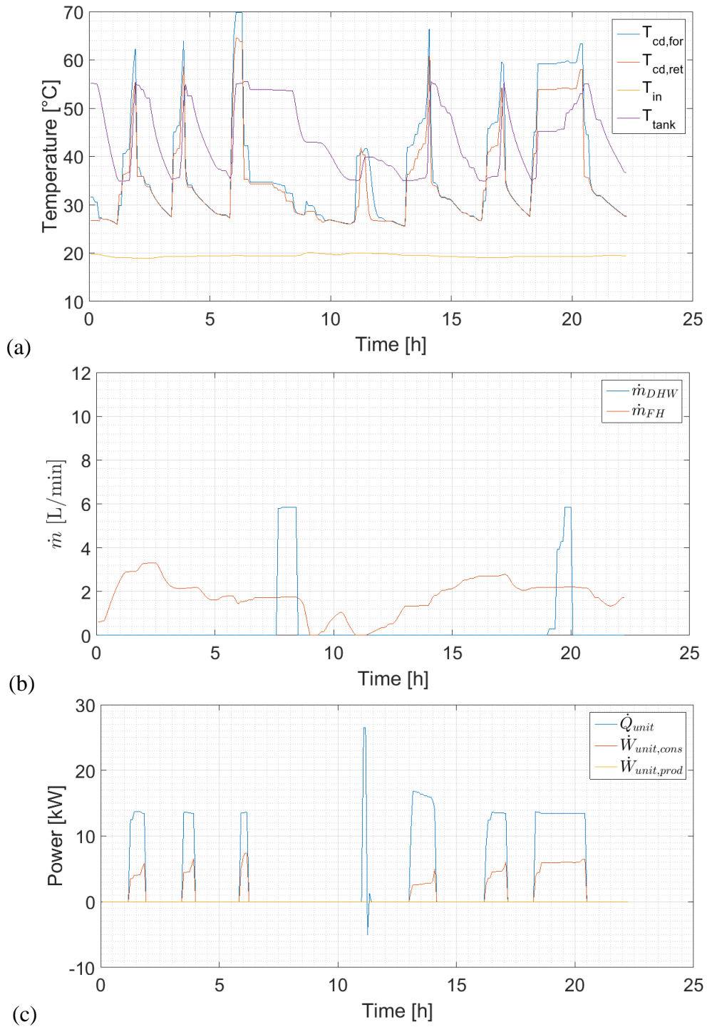
Figure 6 Typical operational conditions of the HP/ORC unit coupled with a DHW tank. T_{cd,for} is HP condenser forward temperature, T_{cd,ret} is the HP condenser return temperature, T_{in} is the indoor temperature inside the house and T_{tank} is the temperature inside the tank at a 0.6m height.
