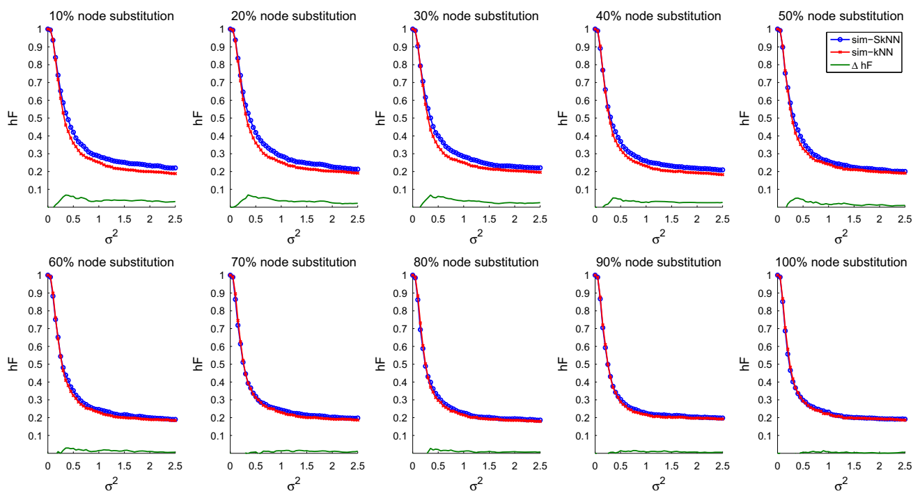
Fig. 10 SkNN vs. kNN results for the second simulation condition, with the substitution perceptual error on the underlying 7-level binary tree taxonomy. Blue and red curves show hF for the hierarchical and
