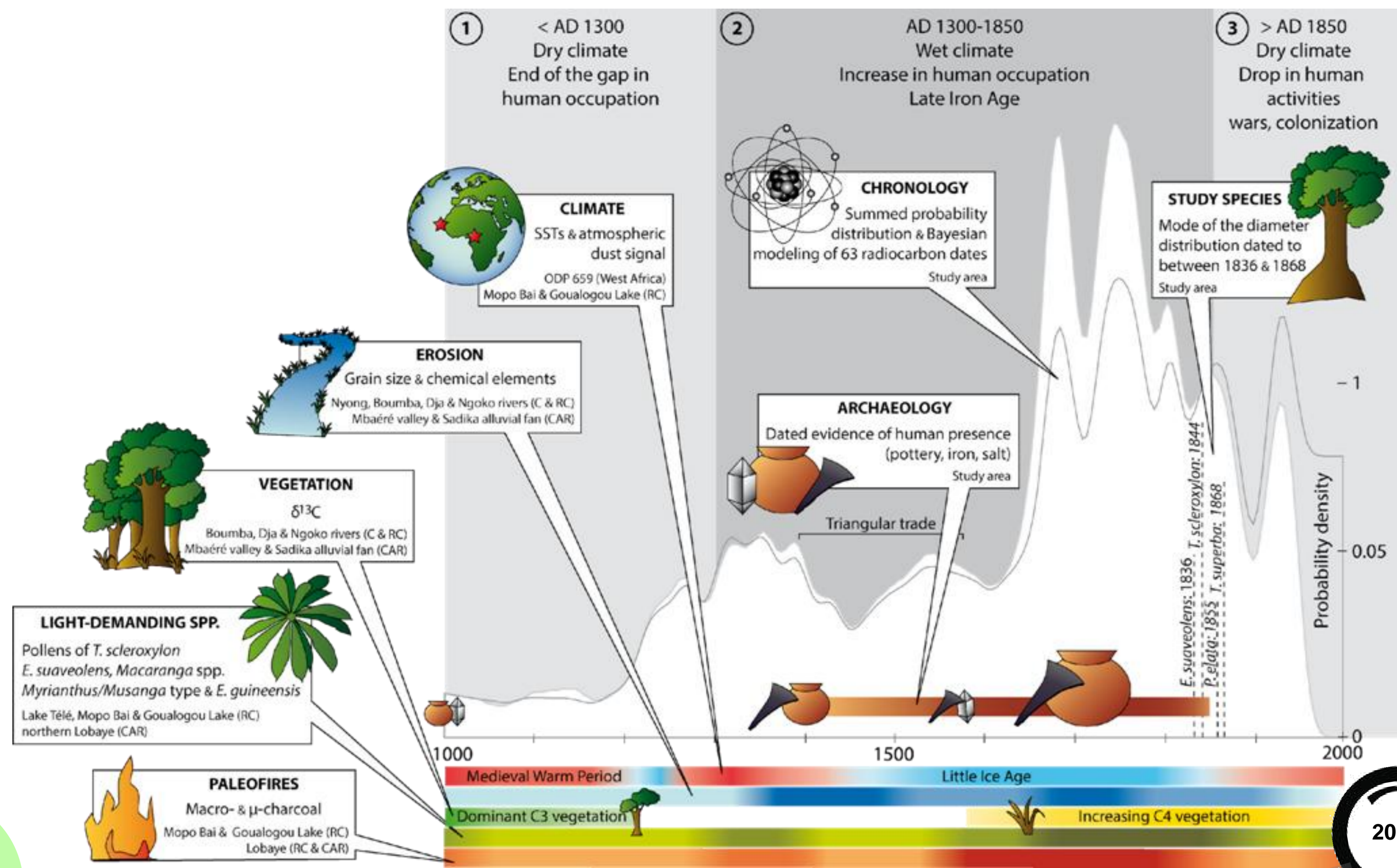
Fig. 1: History of disturbances during the last 1,000 yr in the Sangha River Interval.
