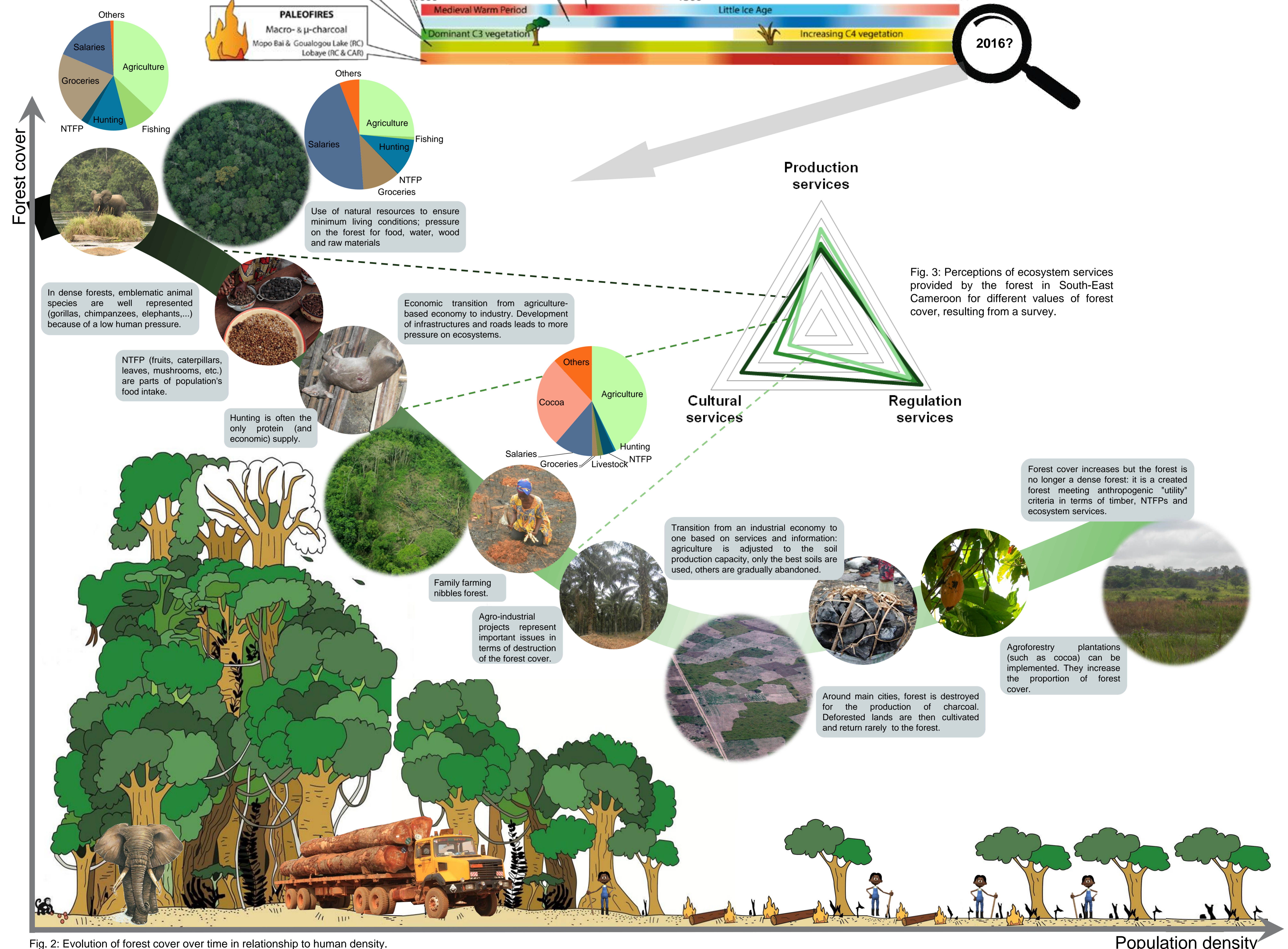
Fig. 2: Evolution of forest cover over time in relationship to human density.
