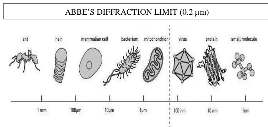
Figure 1. At the end of the 19th century, Ernst Abbe defined the limit for optical microscope resolution to roughly half the wavelength of light, about 0.2 micrometre. This meant that scientists could distinguish whole cells, as well as some parts of the cell called organelles. However, they would never be able to discern something as small as a normal-sized virus or single proteins
