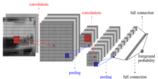
Figure 3. Architecture of our ConvNet for background subtraction.
