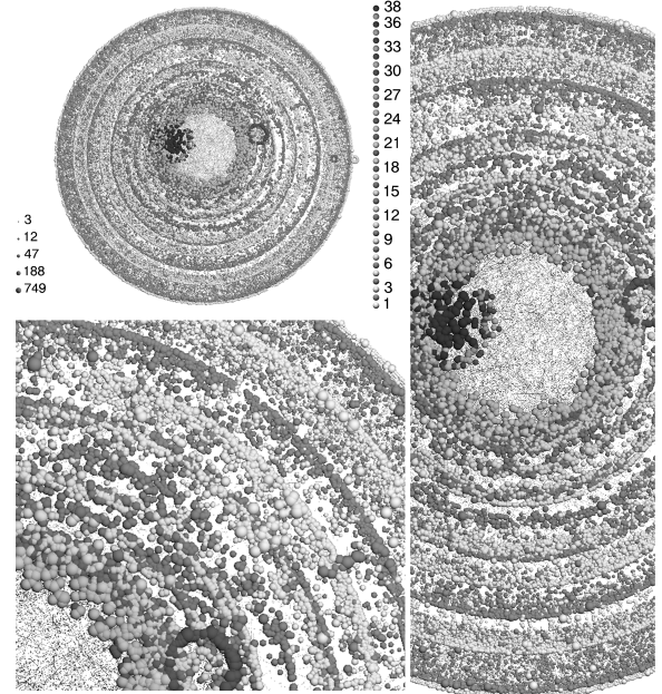
Fig. 6. k -core visualization of router level topology G_r .
