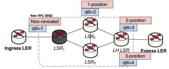
Fig. 2. Example of biased n-position . It shows a scenario where, due to per-packet load balancing issues and the absence of RFC4950 on LSR1 , the n-position could be erroneously inferred: First, traceroute reveals LSR2 (and associates it the 1-position), the next traceroute probe reveals the LH LSR (and associates it the 2-position). Finally, due to load balancing issues on LSR2 the LH LSR is revealed twice (with different qTTL value).
