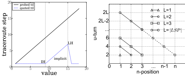
(a) qTTL signature. (b) u-turn signature. Fig. 1. Signatures behavior for implicit MPLS tunnels.
