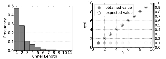
(a) Tunnel length distribution (b) qTTL and n-position comparison Fig. 3. Comparison between obtained and expected values for qTTL and u-turn.
