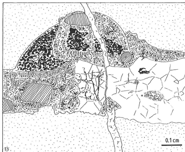
Figure 6. lame mince ULB TP 97.
