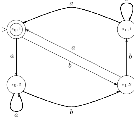
Fig. 3. From generalized Büchi to Büchi
