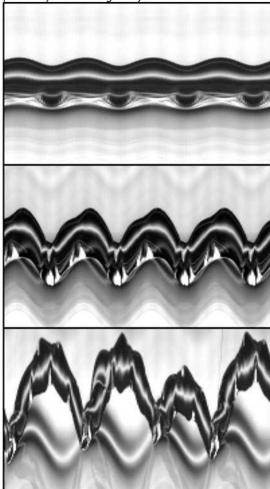
FIG. 1. Successive snapshots of the bouncing droplet have been juxtaposed for \gamma = 0.4 (top), 0.9 (middle), and 1.3 (bottom) times the gravity.
