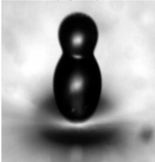
FIG. 2. Peanut shape of the droplet obtained when the acceleration is large ( \gamma=1.3g ) (enhanced online).
