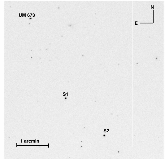
Fig. 1. Part of one Gunn i DFOSC CCD frame of UM 673. The field of view is 5' \times 5' . Two reference stars are indicated (S1 and S2). Star S1, whose absolute photometry is well known (Nakos et al. 2003) has been used to normalize the CCD frames. Star S2 was taken as a comparison star.
