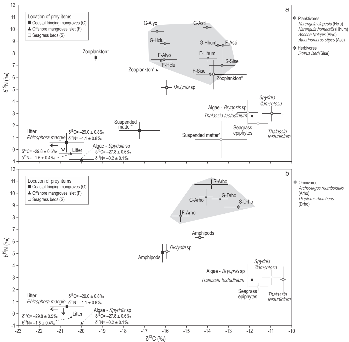
Figure 2. Mean \delta^{13}C and \delta^{15}N values ( \pm standard deviation) of (a) planktivorous and herbivorous fishes and (b) omnivorous fishes (grey areas) and their prey sampled in mangroves and seagrass beds. The asterisks indicate potential prey of planktivorous fishes.
