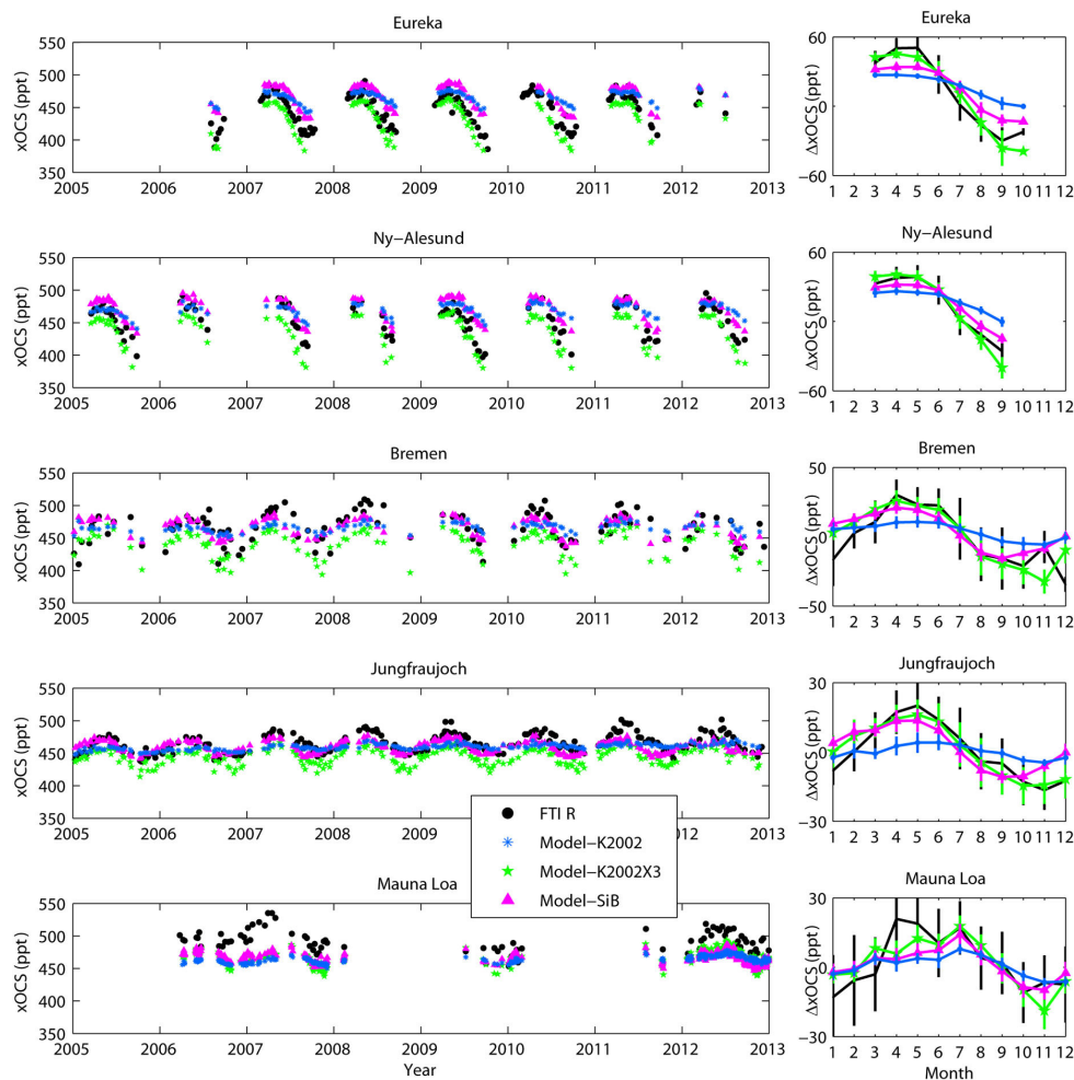
Figure 2. Comparison of FTIR measurements of OCS to model simulations at Eureka, Ny-Ålesund, Bremen, Jungfraujoch, and Mauna Loa. The left panels show weekly means from 2005 to 2012. The right panels are the monthly mean relative xOCS (relative to annual mean) averaged for multiple years. The error bars are the standard deviations of each month. The FTIR retrievals are shown by black dots. The model simulations are driven by K2002 (blue asterisks), K2002x3 (green stars), and SiB (magenta triangles).
