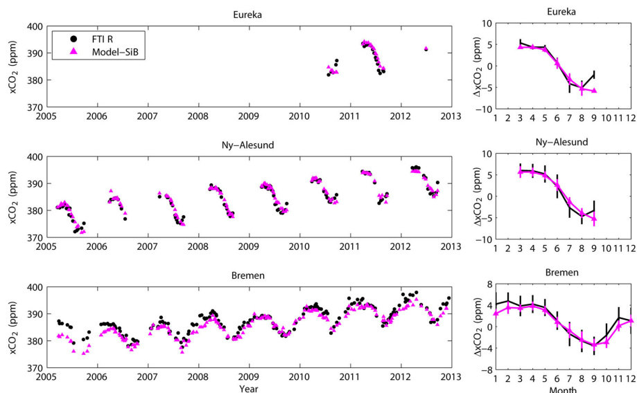
Figure 6. Comparison of FTIR measurements of CO 2 (black dots) to model simulations with SiB land fluxes (magenta triangles) at Eureka, Ny-Ålesund, and Bremen. The left panels show weekly means from 2005 to 2012. The right panels show the monthly mean relative xCO 2 (relative to annual mean) averaged for multiple years. The error bars are the standard deviations of each month.
