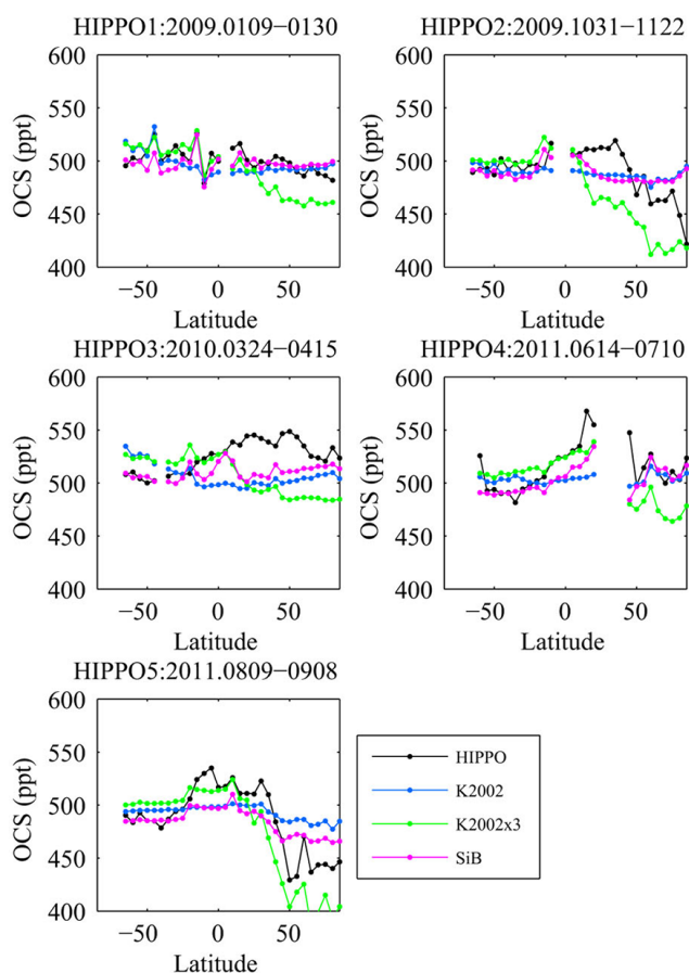
Figure 3. Comparison of HIPPO-OCS measurements and model simulations. The five campaigns are compared separately to show latitudinal gradient in different seasons. To minimize the influence of the stratosphere, only the measurements lower than 9 km are used. The model outputs are selected at the nearest measurement location and time. The measurements and model output are averaged in 5° bins. The HIPPO data are shown by black dots. The model simulations are in the same colors as those shown in Fig. 2.
