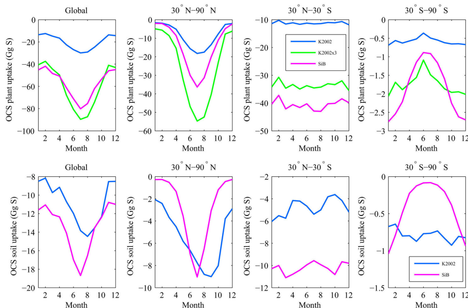
Figure 5. Monthly totals of OCS plant uptake (top) and soil uptake (bottom) of K2002 (blue), K2002x3 (green), and SiB (magenta) for global, 30–90° N, 30° N–30° S, and 30–90° S.
