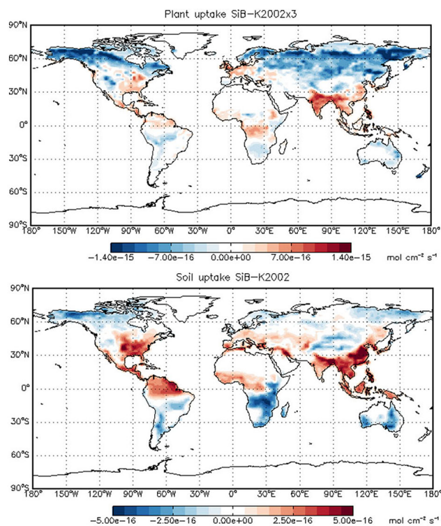
Figure 4. Difference between SiB OCS plant uptake and K2002x3 (top, SiB – K2002x3), difference between OCS soil uptake and K2002 (bottom, SiB – K2002).
