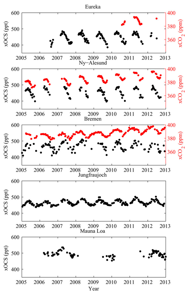
Figure 1. Weekly mean xOCS (black dots) and xCO 2 (red dots) retrieved from FTIR spectra at Eureka, Ny-Ålesund, Bremen, Jungfraujoch, and Mauna Loa.
