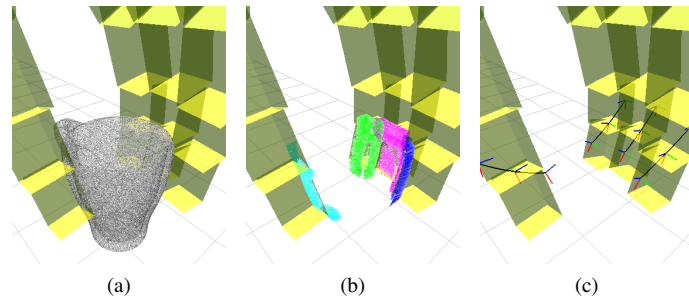
Fig. 5. Example top grasp of a mug represented by a point cloud (panel a). The dotted regions are rays between features and the closest hand link surfaces (panel b). The black curves with frames at the fingertips represent the range of hand configurations in Eq. (16) (panel c).
