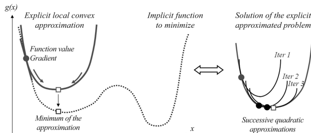
Fig. 4. Illustration of the Sequential Convex Programming approach
