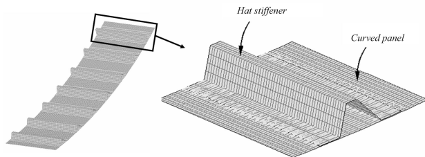
Fig. 8. Curved composite panel and its super-stiffeners
