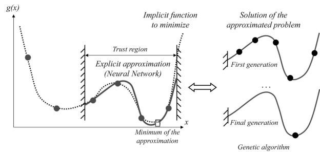
Fig. 5. Illustration of the Surrogate Based Optimization approach
