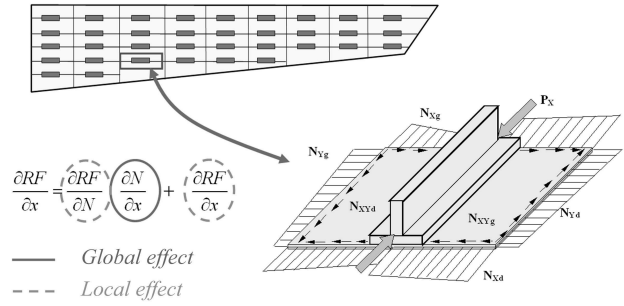
Fig. 3. The bottom surface of a wing and its associated super-stiffeners where local computations are carried out
