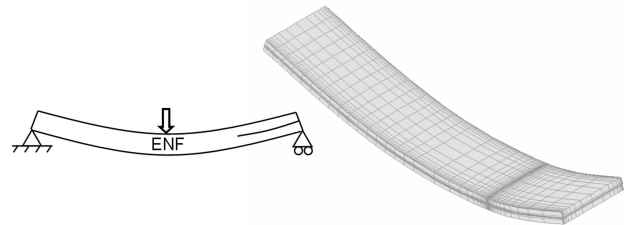
Fig. 6. The ENF test case, and its finite element model
