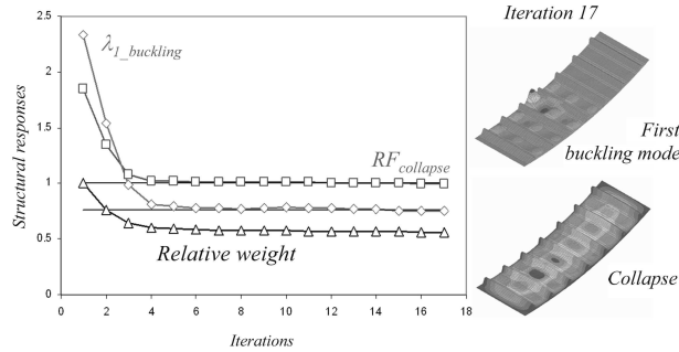
Fig. 10. Convergence history for buckling and collapse optimization
