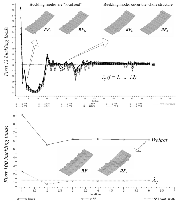
Fig. 9. Convergence history for 12 and 100 buckling modes
