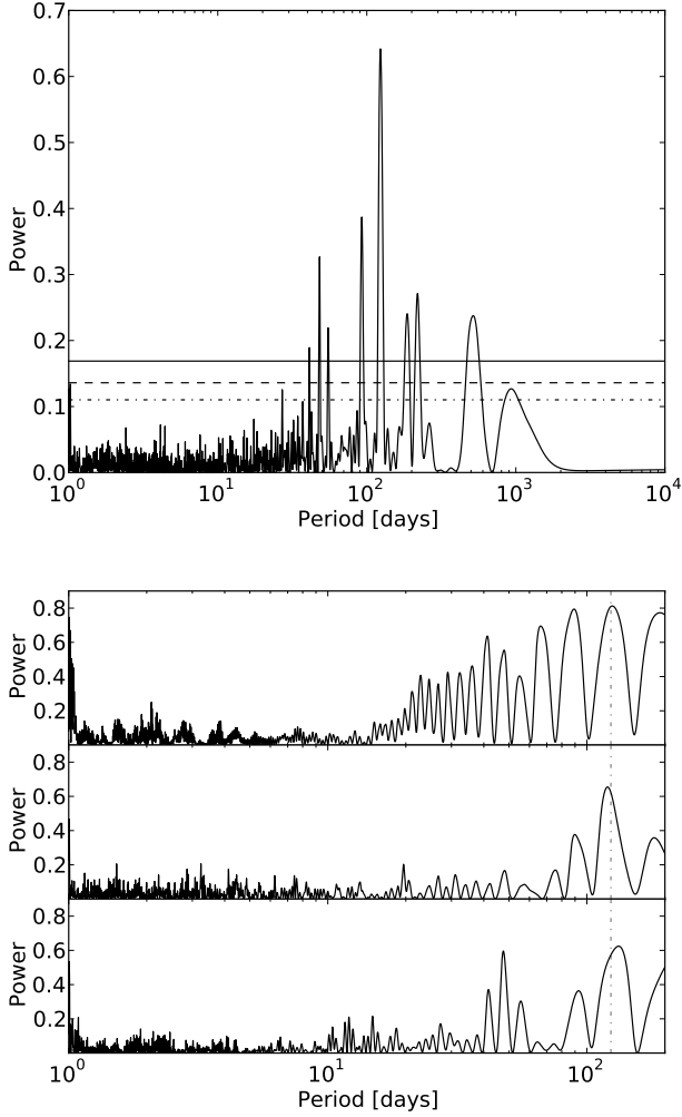
Fig. 3. Top panel: Periodogram of the residuals from the subtraction of the first keplerian ( P=30.6 d). The horizontal lines have the same meaning as in Fig. 2. Bottom panel: Periodogram. We split for subsets of the observational epochs, defined in the caption to Fig. 2; in spite of the poor sampling of some of the subsets for a 123 d period, all show a peak around this period.
