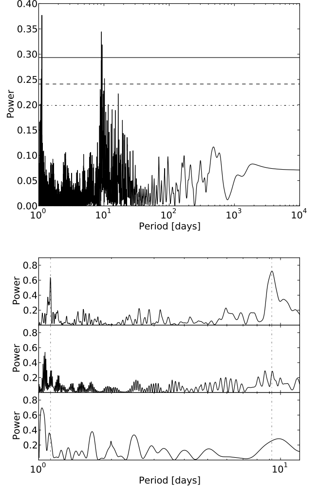
Fig. 10. Top panel: Periodogram of the radial velocities of GJ 3543. The horizontal lines represent the same false alarm levels as in Fig. 2. The two peaks at 1.1 and 9.2 d have less than 0.3% FAP. Bottom panel: Periodograms for three independent subsets of observation epochs (BJD-2400000=55500-55750, first row; 55850-56050, second row; 56340-56380, third row). The 1.1 and 9.2 d peaks (marked by vertical dashed-dotted lines) are both unstable over time.
