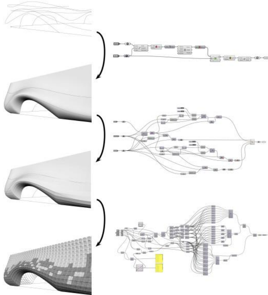
Fig. 1. Evolution of the parametric model [5]
