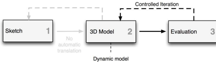
Fig. 2. Parametric modeling process
